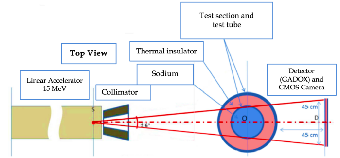
FIGURE 2: FORESEEN X-RAY RADIOLOGY SYSTEM FOR PLINIUS-2 FR TEST SECTION
