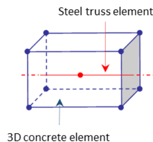
Fig.1 General presentation of the simulation using steel 1D truss and concrete 3D concrete elements.
