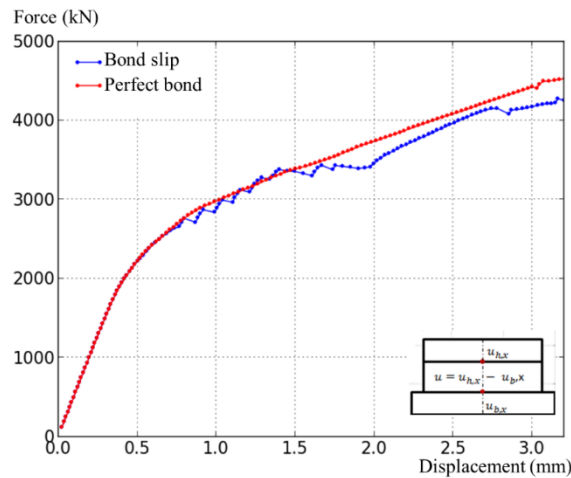
Fig. 16. Evolution of the force as a function of a relative horizontal displacement computed in the middle of the wall
