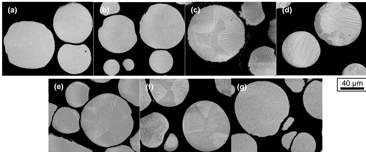
Figure 3: U(Mo) particles microstructure, observed by SEM (BSE mode) in (a) EMP-711, (b) EMP-717, (c) EMP-803, (d) EMP-819, (e) EMP-828, (f) SF-202, (g) SF-402 plates.
