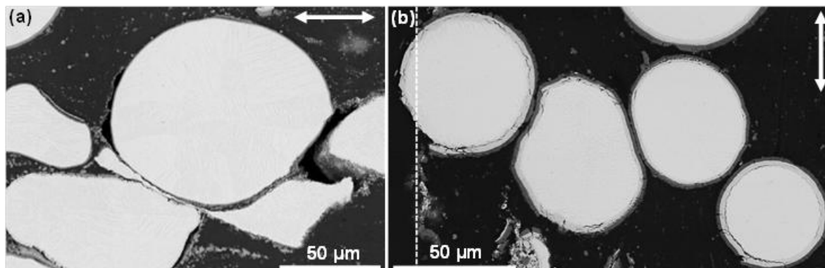
Figure 5: SEM micrographs taken on cross-sections of (a) EMP-828, (b) EMP-819 plates (white arrows: rolling direction - dashed line: approximate location of fuel-cladding interface).
