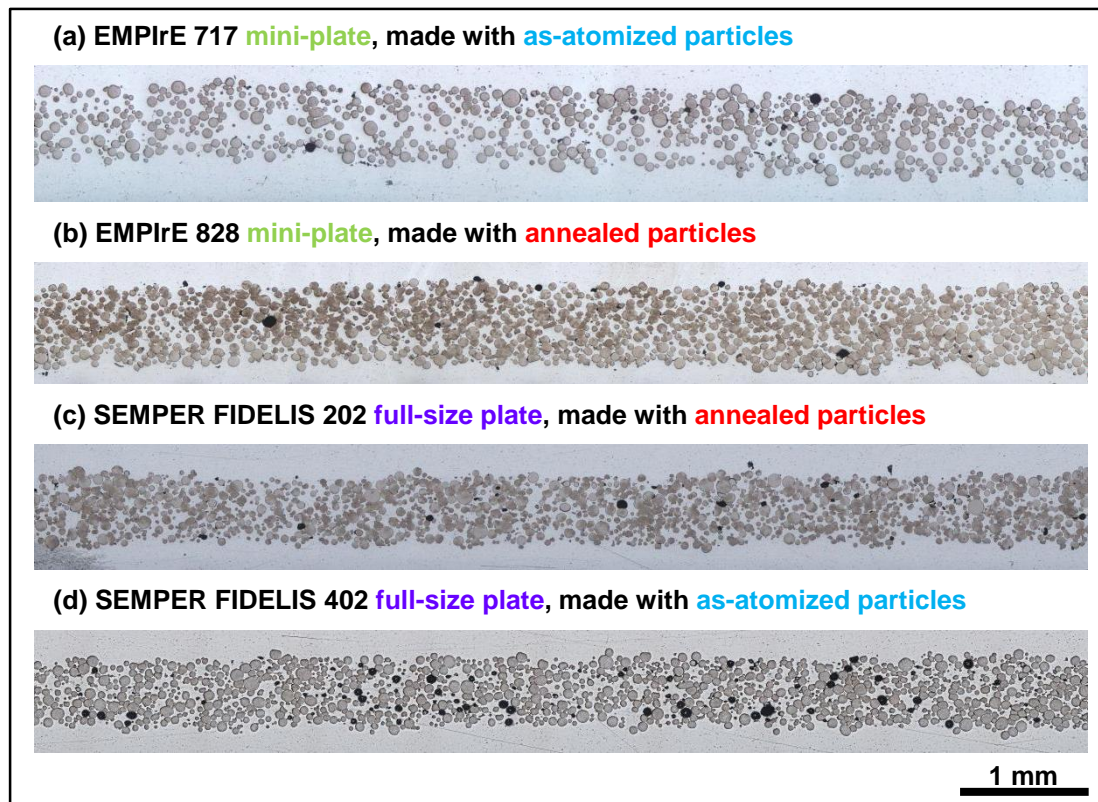
Figure 2: OM macrographs of (a) EMP-717, (b) EMP-828, (c) SF-202, (d) SF-402 plates.
