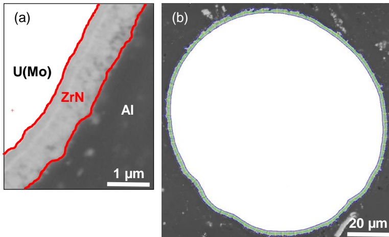
Figure 1: Principle of ZrN coating thickness measurement, on BSE images:
