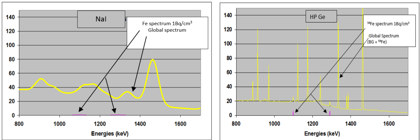
Figure 8 : ^{59}\text{Fe} in the global spectrum with 1\text{Bq}/\text{cm}^3 -Comparison between NaI and HP-Ge Detector
