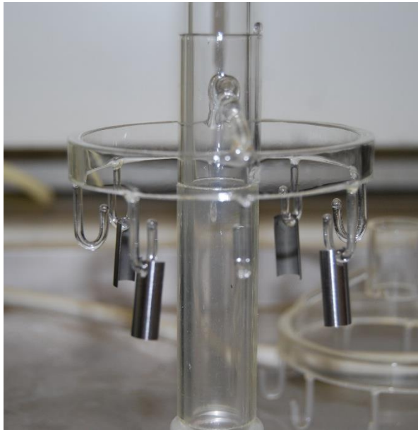
Corrosion coupons hung up on a circular sample holder
