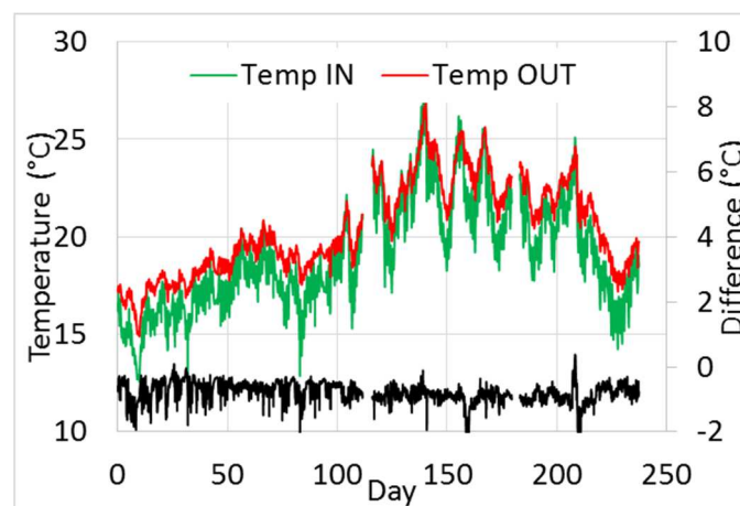
Figure 8: Record of temperature in and out irradiation chamber during the experiment
