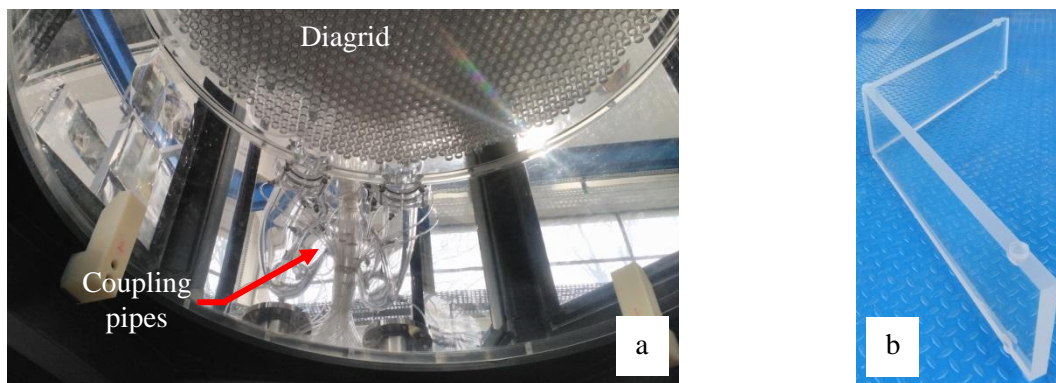
Fig. 4 Bottom view of the MILIPOSO model (a) and diagrid splitting wall (b).
