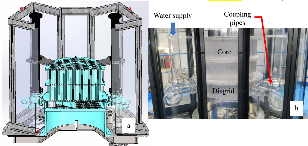
Fig. 3 Cut view (a) and front side (b) of the MILIPOSO mock-up.
