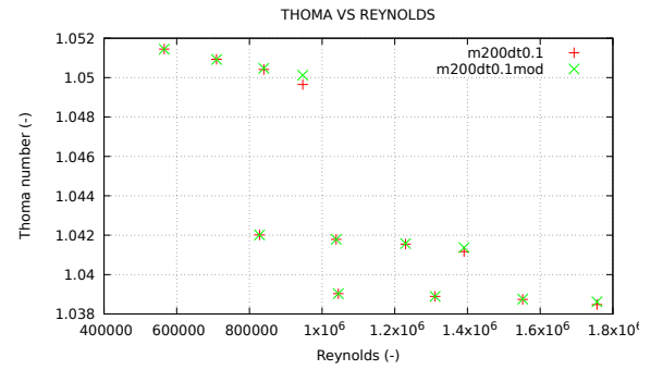
Figure 8. \sigma -Re model sensitivity
