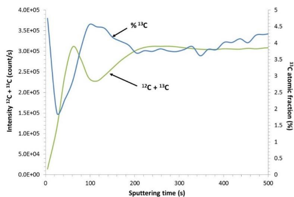
Fig 6. Carbon intensity and 13 C enrichment of C measured through 9Cr surface after corrosion test 9Cr-49CO 2 -1CO 2
