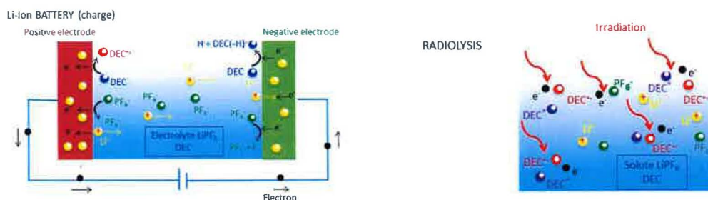
Fig. 1. Comparison between primary electron transfers at the electrodes in the electrolytic charge/ageing processes of a Li-ion battery (in LiPF 6 1 M/diethylcarbonate solution as a model electrolyte) (left), and after ionization in the bulk during radiolysis with the same medium (right) 3 .
