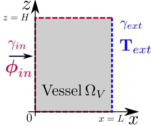
Figure 1: Notations for the vessel discretization
