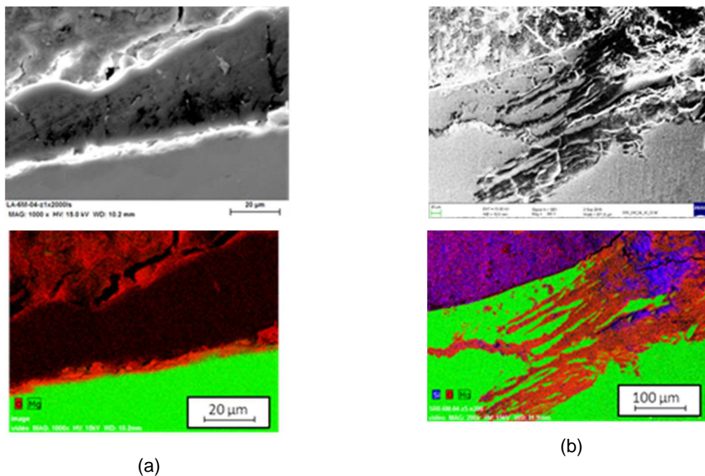
Figure 1: SEM images coupled to EDS for Mg-1.2%Mn alloy in galvanic corrosion assembly embedded for 6 month in (a) the AAS mortar and (b) the SR0 OPC mortar (Green for Mg element – Red for O element – Blue for Si)
