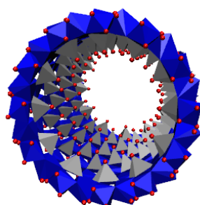
Figure 1 : Imogolite structure. Hydrogens are omitted, Oxygen as red dots, Silicon as grey tetrahedra and Aluminium as blue octahedra.
