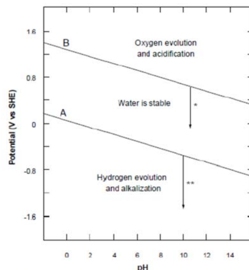
Figure 13 Thermodynamic stability of water, oxygen, and hydrogen. (A is the equilibrium line for the reaction: H_2 = 2H^+ + 2e^- . B is the equilibrium line for the reaction: 2H_2O = O_2 + 4H^+ + 4e^- . * indicates increasing thermodynamic driving force for cathodic oxygen reduction, as the potential falls below line B. ** indicates increasing thermodynamic driving force for cathodic hydrogen evolution, as the potential falls below line A.)
