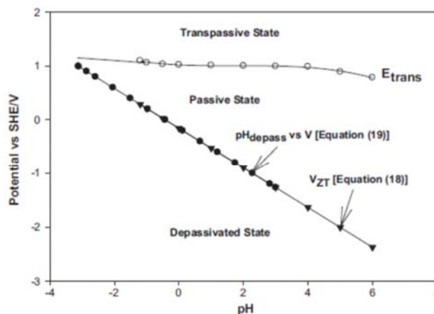
Fig. 9. Primitive Kinetic Stability Diagram (KSD) for Alloy X in 6.256 m NaCl at 50 °C.
