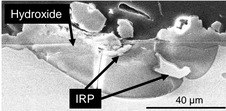
Cross section of a pit (SEM)
