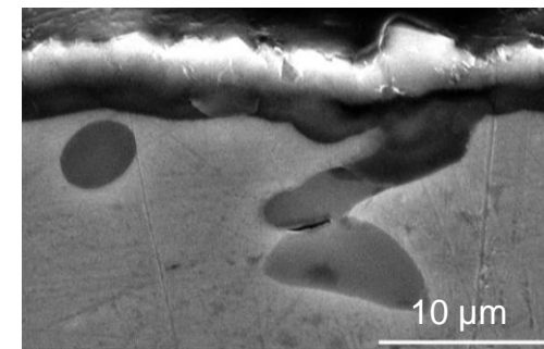
Cross section of Mg_2Si (SEM)
