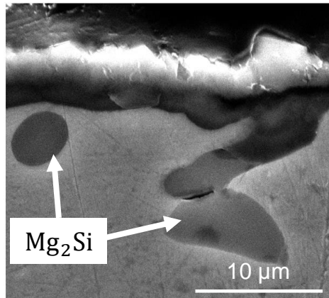
Cross section of Mg_2Si (SEM)
