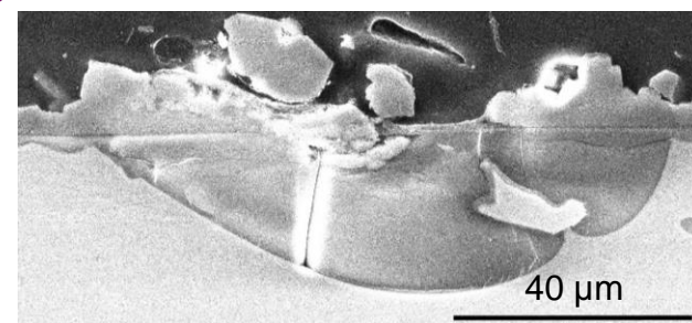
Cross section of pit (SEM)
