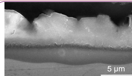
Cross section of aluminium hydroxide of uniform corrosion (SEM)
