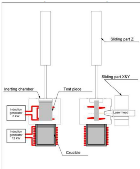
Figure 31: BALHAZAR laser test facility
