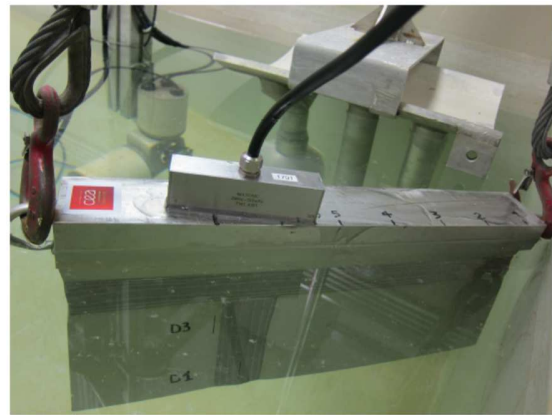
Figure 18: Core supporting skirt mock-up, during water tests
