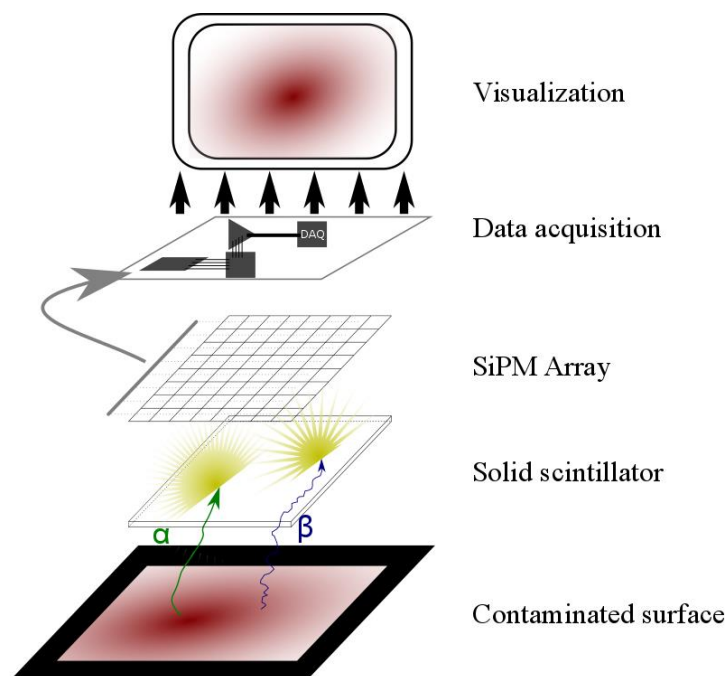
Figure 1: Schematic view of the MAUD detector
