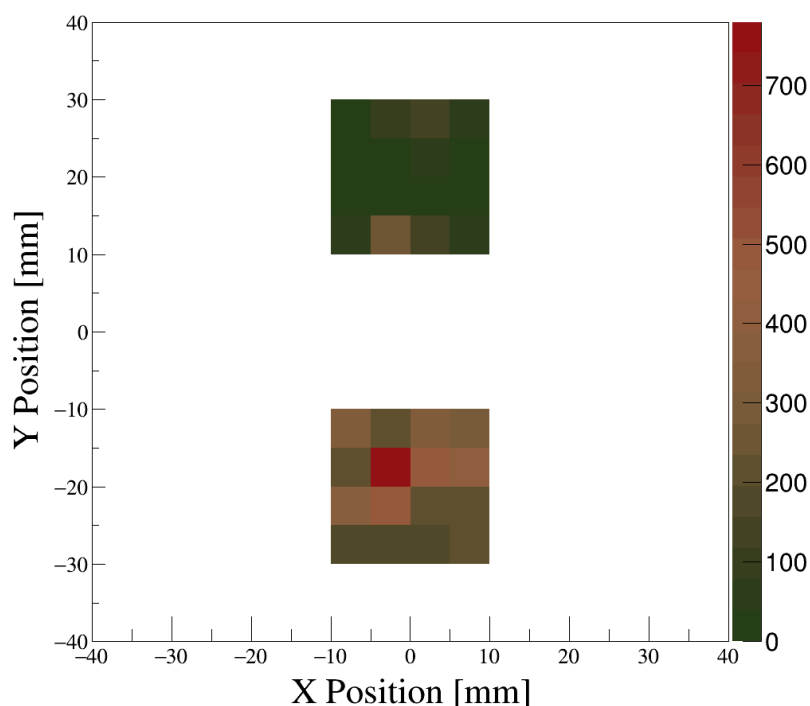
Figure 2: Position mapping using ^{36}\text{Cl} beta source
