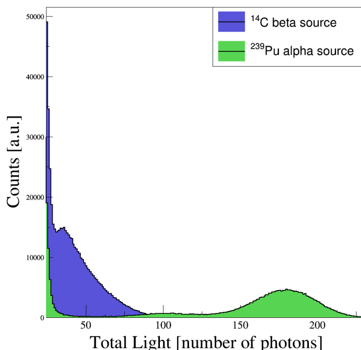
Figure 3: Characterization of beta and alpha source
