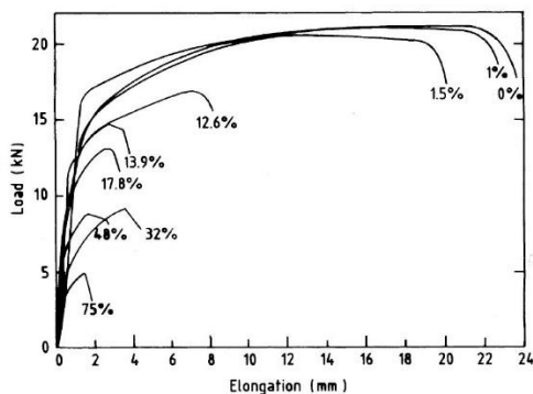
Figure 2: Evolution of corroded steel bars ductility [16]
