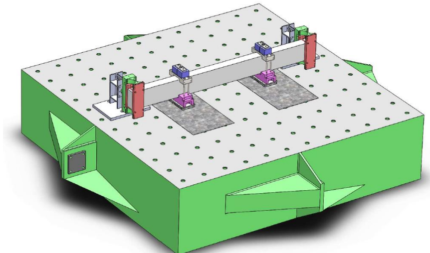
Figure 13: General view of the experimental setup for dynamic tests
