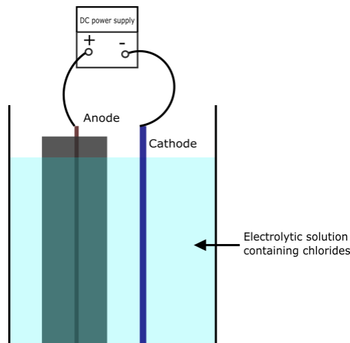
Figure 1: Set-up for accelerated corrosion by imposed current
