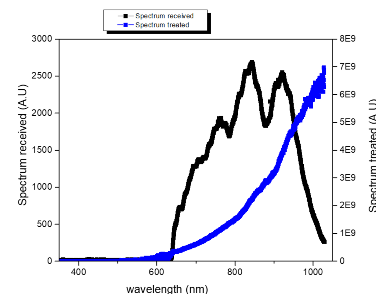
Spectrum as received from the spectrometer of a UO 2 pellet heated at 1200°C (black) and after processing with the inverse transfer function (blue)
