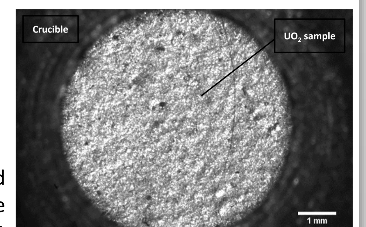
Observation of a UO 2 pellet with the optical system
