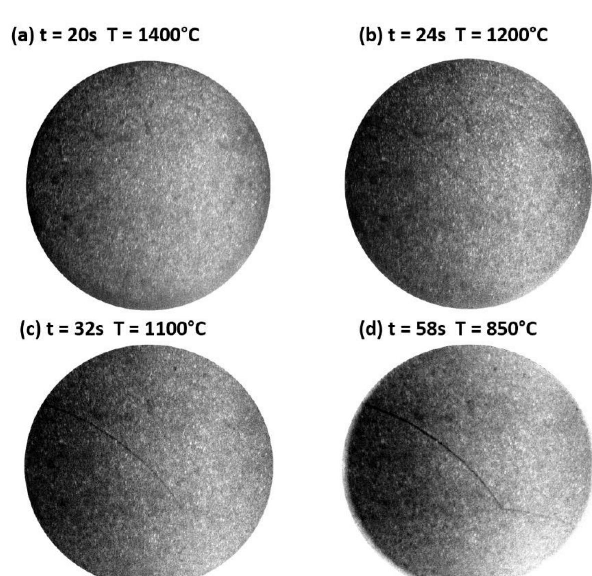
Image sequence illustrating the cracking of the pellet during a cooling phase
