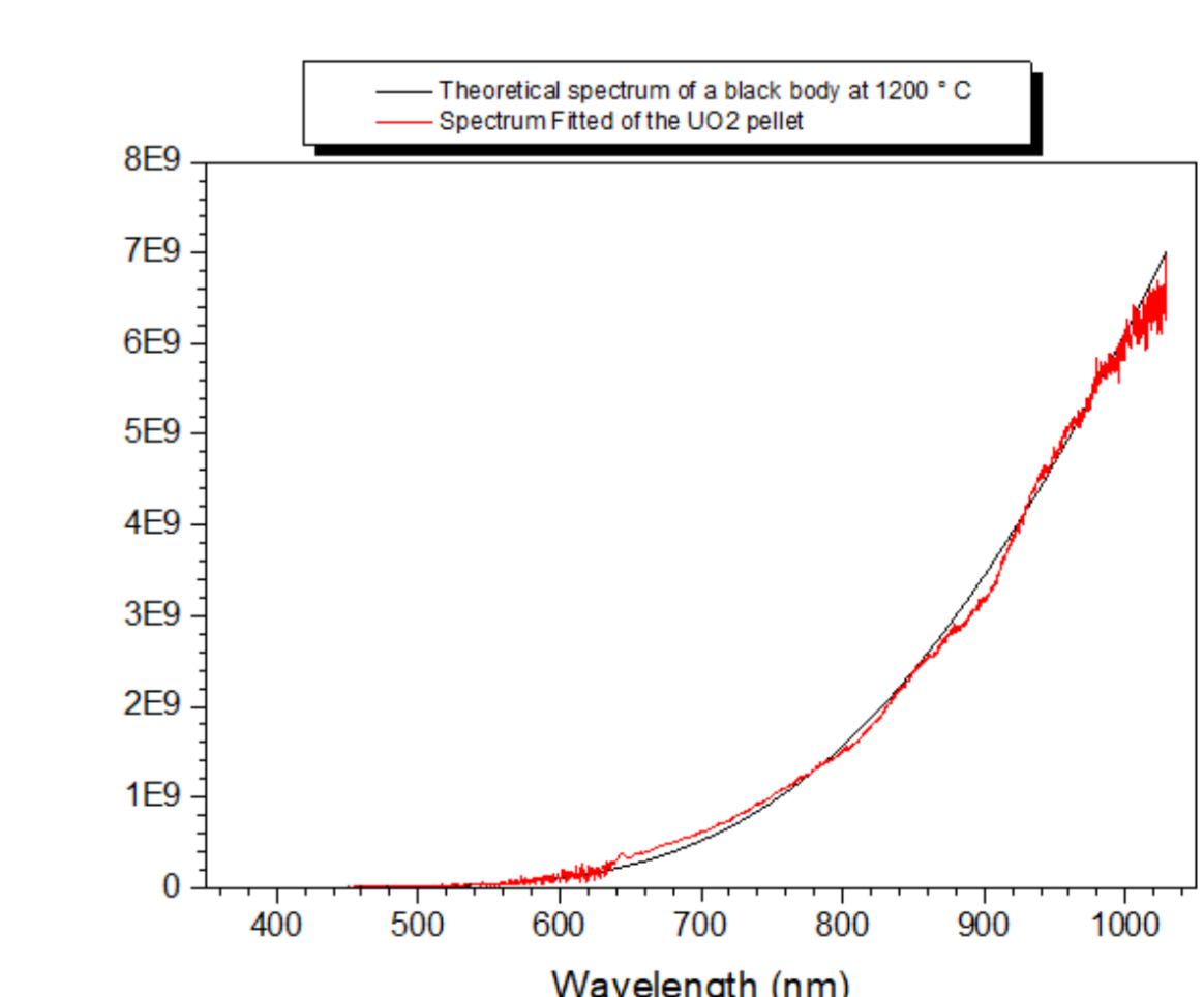
Measured spectrum of a heated UO 2 pellet (red) and fitted with Planck's law at 1200°C (black)
