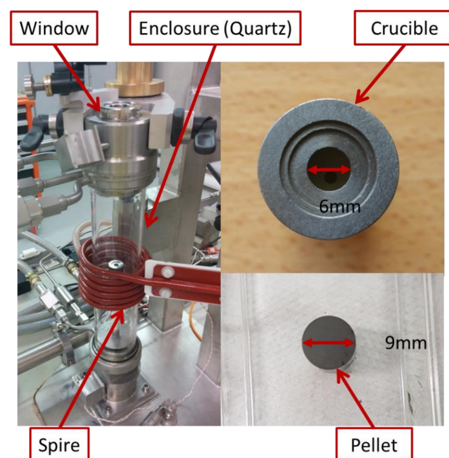
Schematic and photo of the optical device operating on the Merarg mock-up experiment
