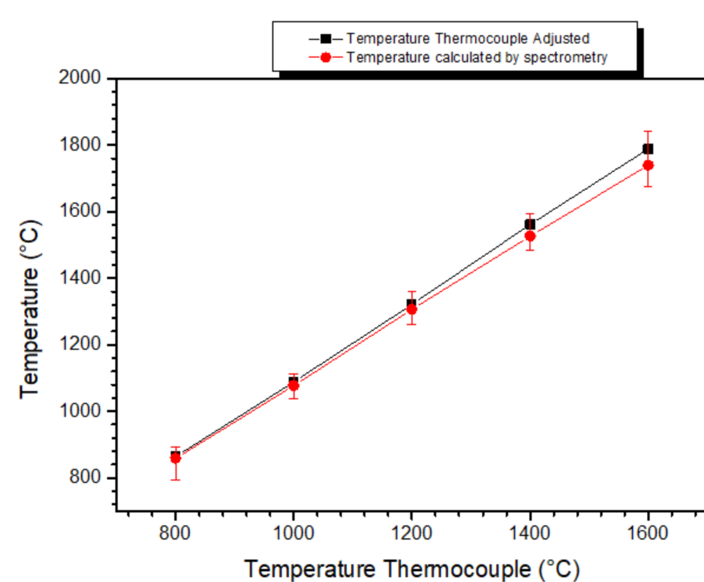
Temperature of the sample from the qualification phase and, as determined, by multispectral pyrometry
