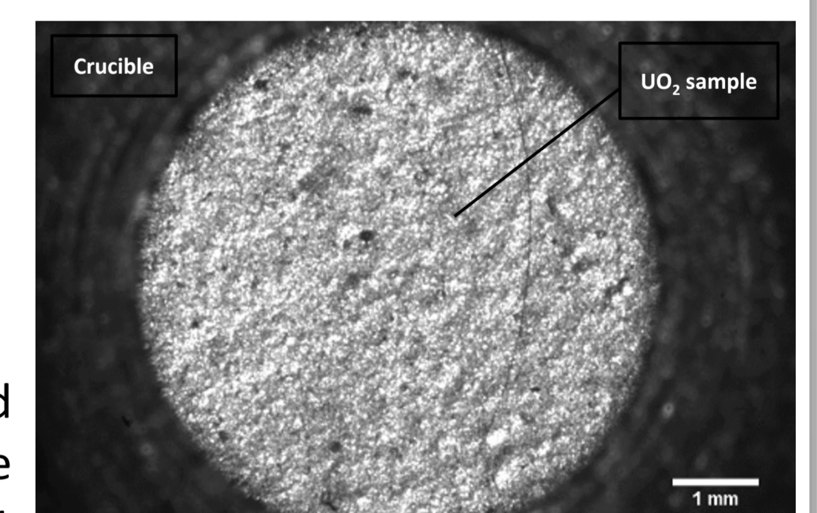
Observation of a UO 2 pellet with the optical system
