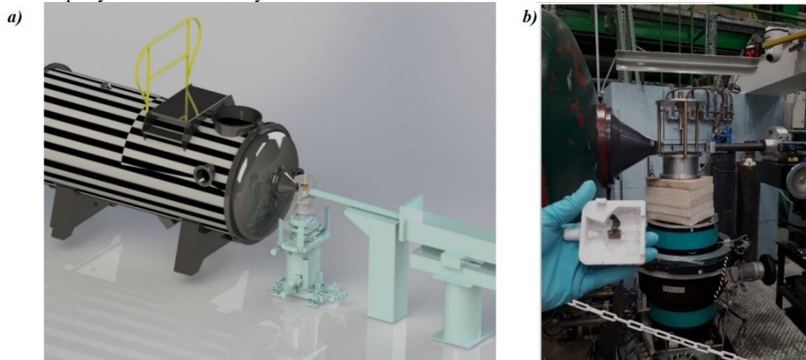
Figure 1 : a) 3D model of the implementation of a low field NMR spectrometer on the LLB SANS instrument PAXY – the one-sided NMR magnet is seen in the middle of the drawing between the neutron guide (in turquoise blue) and the neutron detector box (zebra) (courtesy P. Lavie). b) Real picture of the central part and the NMR-Neutron probehead.
