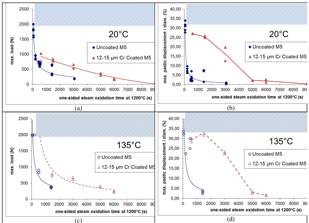
Fig 2: Post-Quenching Ring Compression Test properties evolution as a function of steam oxidation time at 1200°C [6]
