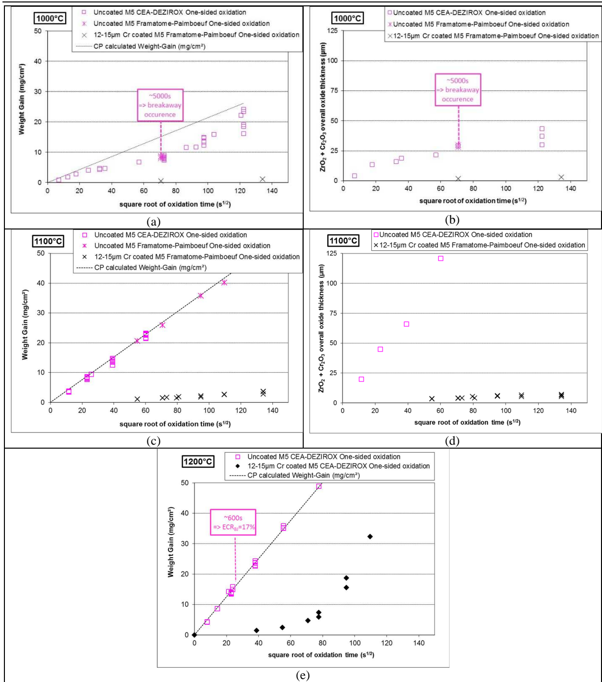
Fig 1. Evolution of weight gain and of overall oxide thickness of uncoated and 12-15µm Cr coated M5 cladding segments as a function of the square root of the steam oxidation time
