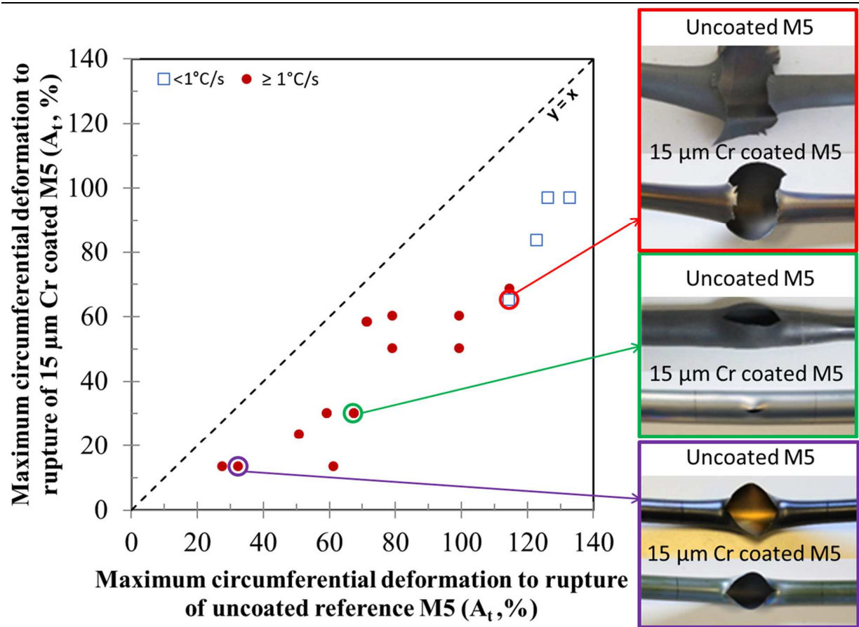
Fig 3. Maximum circumferential deformations ( A_t ) for Cr coated M5 compared to those measured for uncoated references, tested in the same conditions (Temperature range: 0.1^\circ\text{C/s} to 25^\circ\text{C/s} , Pressure range: 10 to 100 bars)
