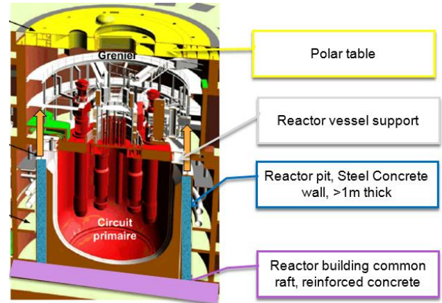
Figure 8. Steel Concrete Reactor pit (in blue) in the reactor vessel environment (© CEA-FRAMATOME-BOUYGUES)
