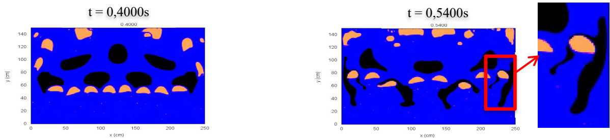
Figure 9. Time evolution for t \leq 0,54s for VF-U1 simulation. Black, orange and blue colors represent metal, gas and oxide phase respectively
