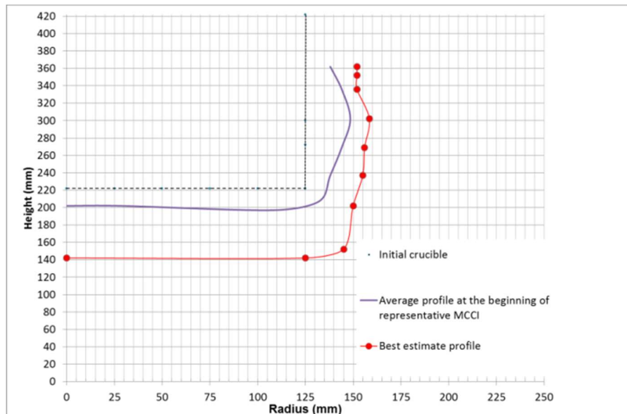
Figure 3. Initial (dotted black line) and final ablation (red line with dots) profiles of the representative MCCI phase in VF-U1 test
