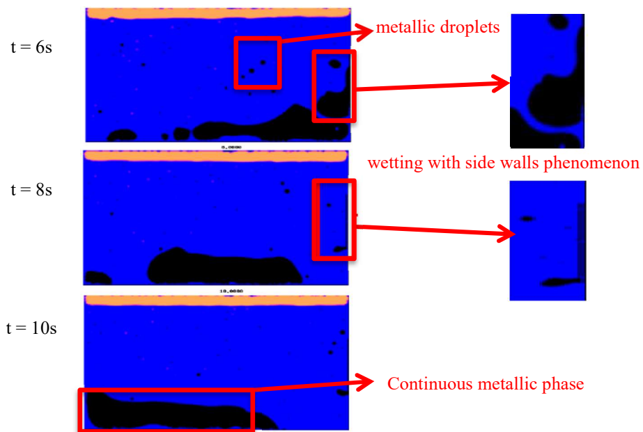
Figure 10. Snapshots of VF-U1 simulation for 6s < t < 10s . Black, orange and blue colors represent metal, gas and oxide phase respectively
