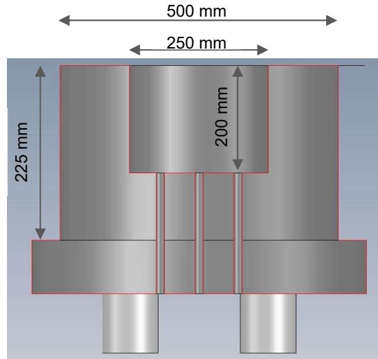
Figure 1. Overview of VF-U1 test section.
