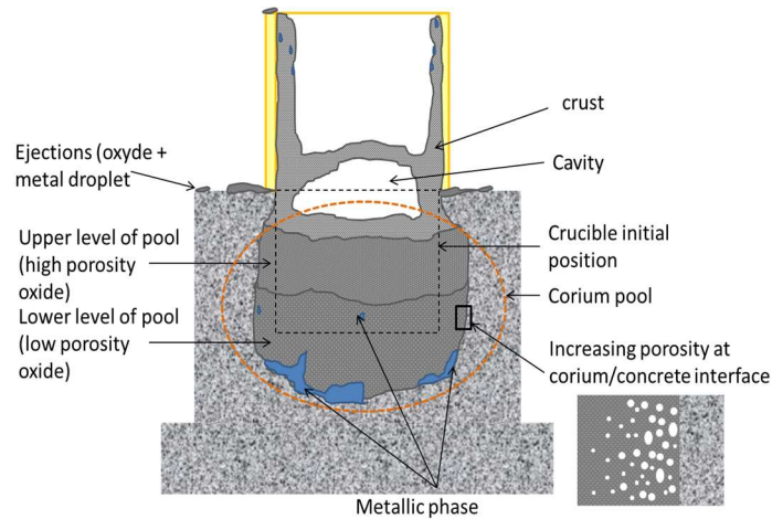
Figure 4. Topology of the frozen melt
