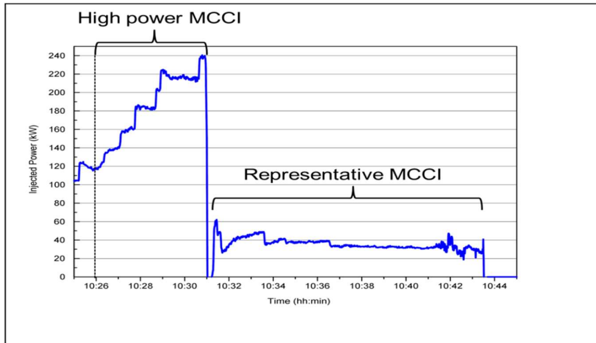
Figure 2. Injected power into the melt during the MCCI phase of VF-U1
