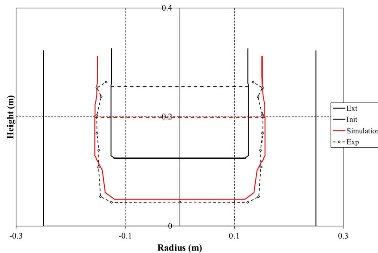
Figure 6. : Initial and final ablation profiles calculated with MCCI-Code and comparison to the experimental profile
