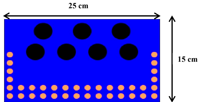
Figure 8. Initial repartition of the 3 phases used in the numerical simulations (gas bubbles in orange, metal drops in black and the oxidic phase in blue)
