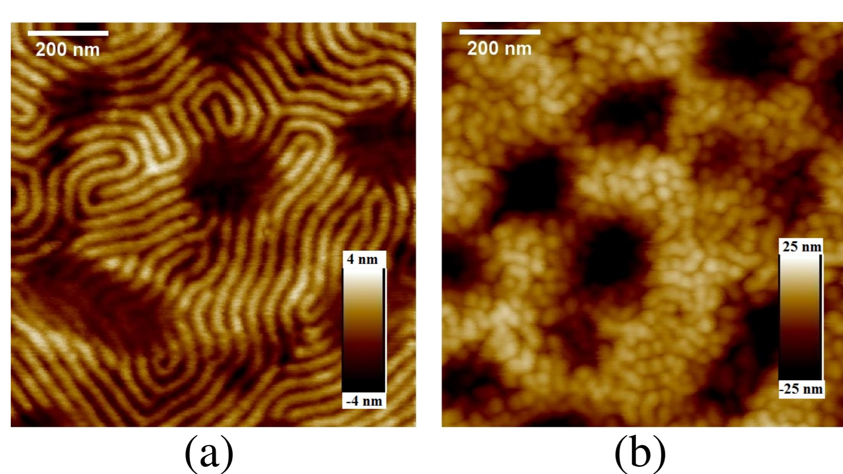
Figure 3: AFM height pictures of deposited and annealed PS- b -P2VP film a/ without and b/ with AuNPs formed by sonication. The presence of the AuNPs inside the cylinders triggers their re-orientation almost normal to the substrate.
