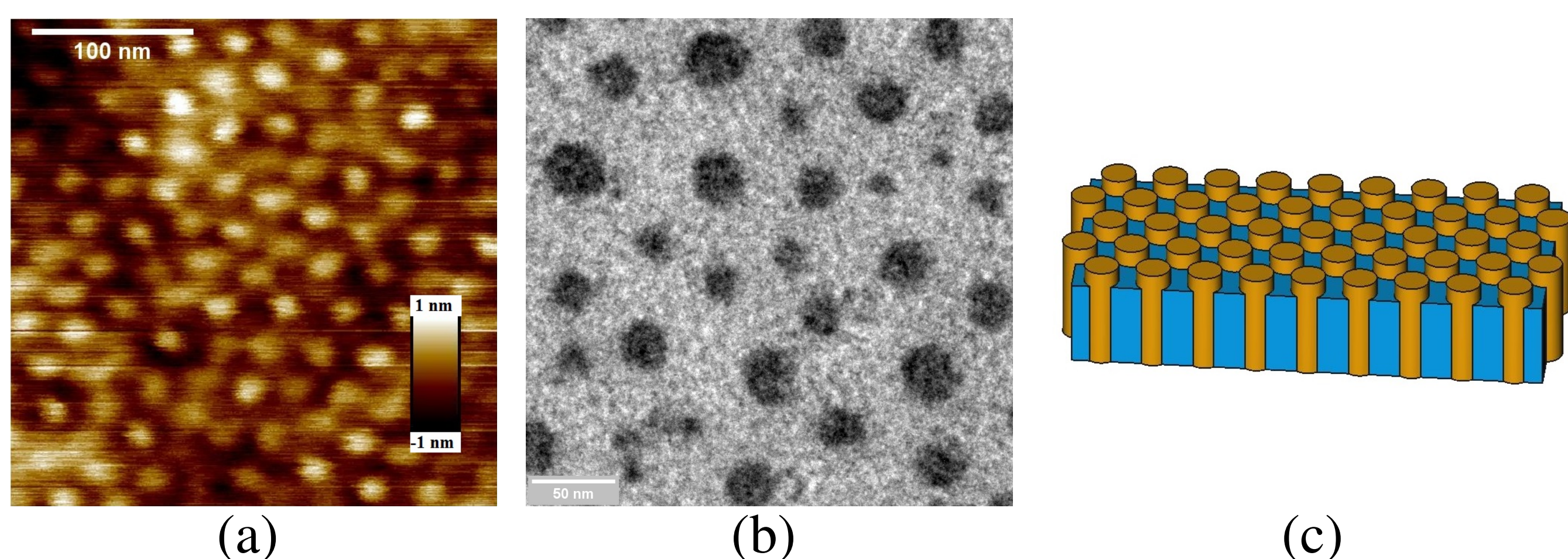
Figure 1: a/ AFM height picture and b/ TEM picture of PS- b -P4VP cylinders oriented normal to the silicon substrate after spin-coating. The cylinders have a 2D-hexagonal organization and their average diameter is 40 nm; c/ 3D-illustration of the cylinders of PVP (orange) in the PS matrix (blue) with an orientation normal to the substrate and a hexagonal organization.
