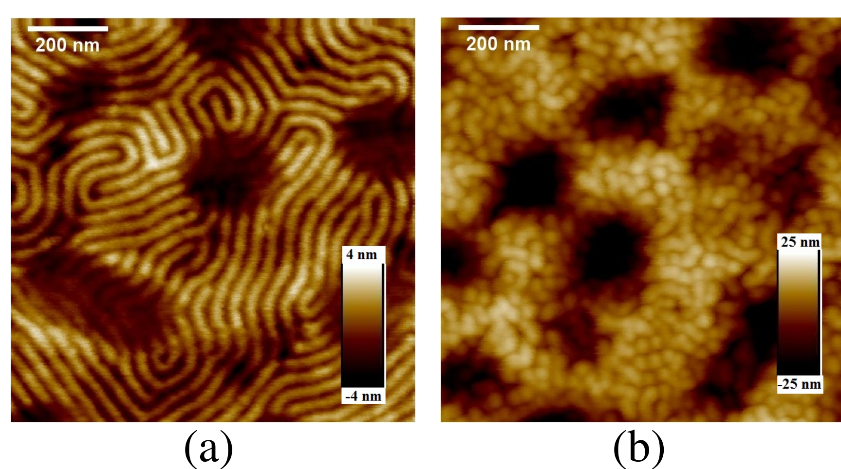
Figure 3: AFM height pictures of deposited and annealed PS- b -P2VP film a/ without and b/ with AuNPs formed by sonication. The presence of the AuNPs inside the cylinders triggers their re-orientation almost normal to the substrate.
