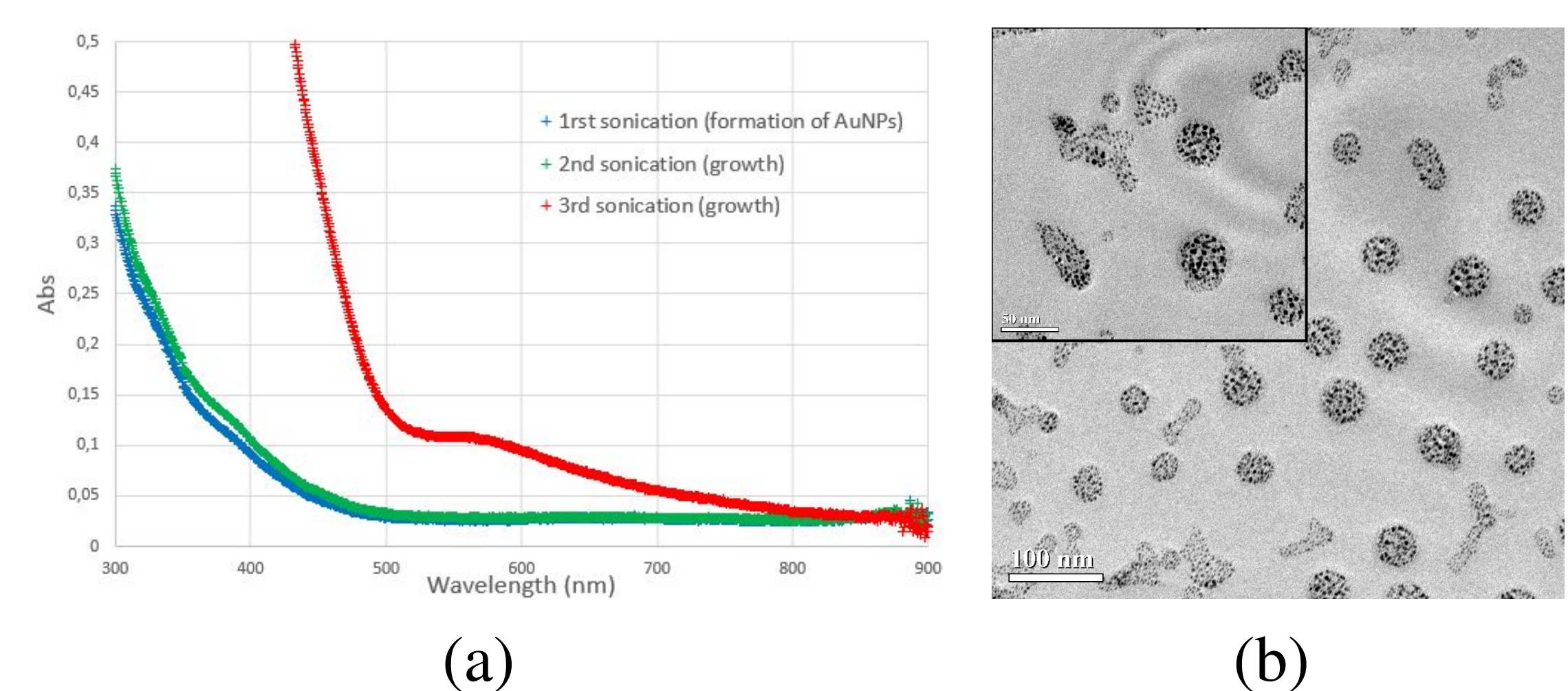
Figure 4: a/ UV-visible spectra: after the formation of AuNPs (blue) and the first addition/sonication (green), no plasmon is noticed. The plasmon peak (around 560 nm) appears after the second addition/sonication; b/ TEM picture of the film for a AuNPs/PS- b -P4VP solution after formation and growth of the AuNPs. The AuNPs are larger (3-4 nm, see inset), which explains their plasmon resonance and still located inside the cylinders. The amount of gold by pyridine is 10 equivalents and each growth step adds 2 more equivalents (for a total of 2 steps).
