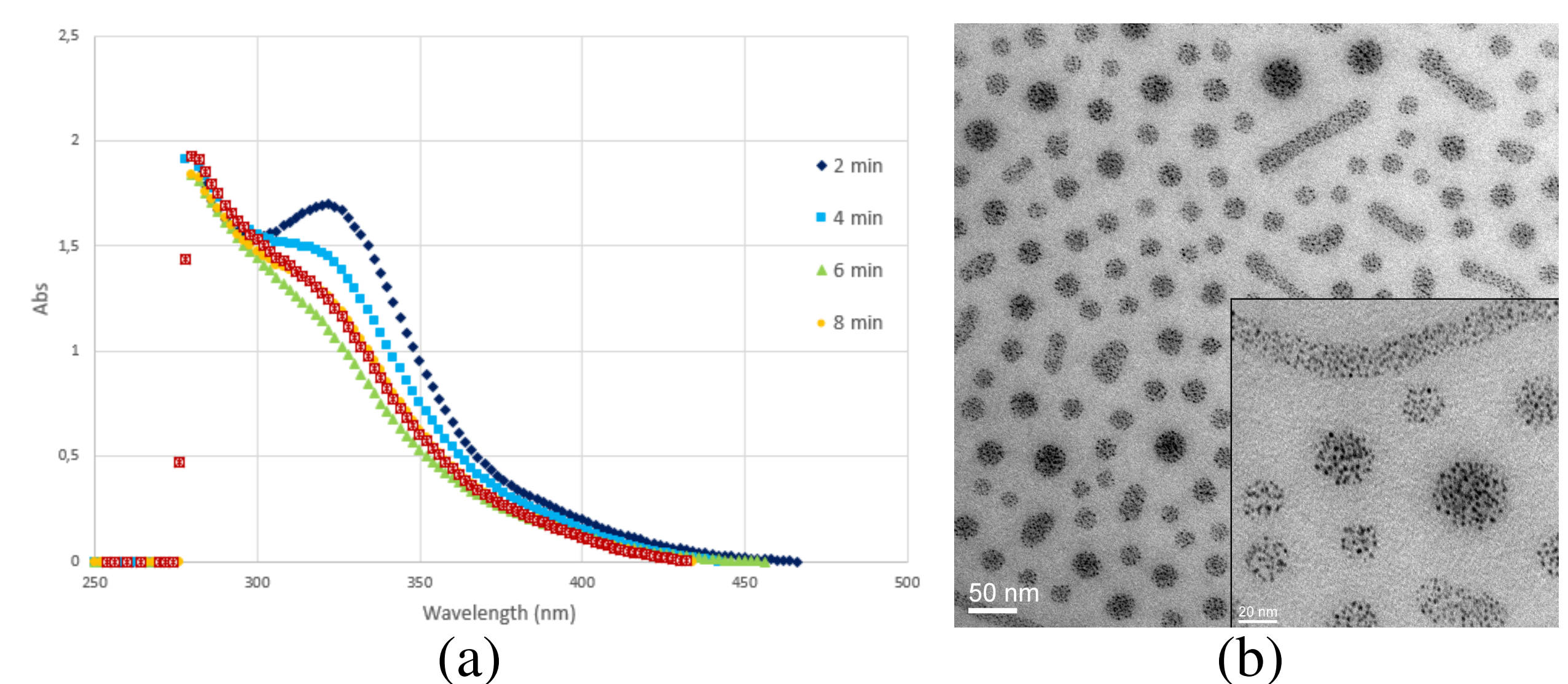
Figure 2: a/ UV-visible spectra showing the decrease of the gold salt peak over the sonication; b/ TEM picture of AuNPs formed by sonication and confined in PS- b -P4VP cylinders oriented normal to the substrate. The AuNP size is around 2 nm (see inset). The amount of gold per pyridine is 5 equivalents.
