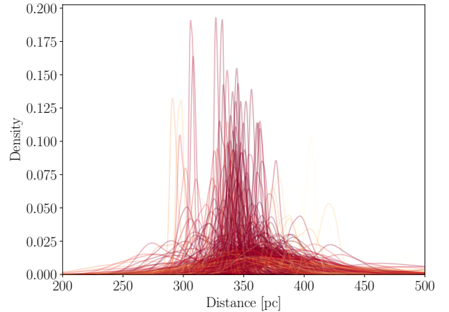
Fig. 10. Individual posterior distance distributions of the members of the GDR2 analysis computed with the Kalkayotl code.
