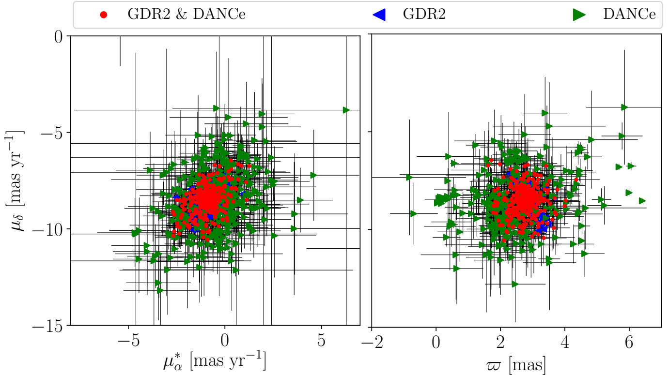
Fig. 6. Vector point diagram ( left ) and parallax–proper motion diagram ( right ) of the IC 4665 open cluster. The members are shape- and colour-coded according to their origin: GDR2 and DANCe analysis (red circles), only GDR2 analysis (blue left-pointing triangle), and only DANCe analysis (green right-pointing triangle).
