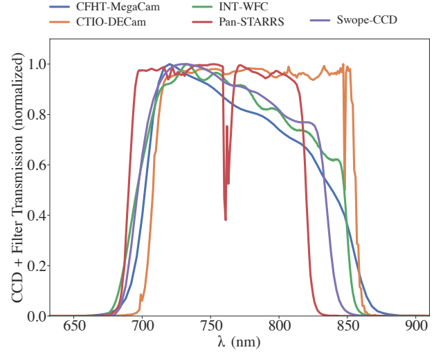
Fig. 2. Transmission curves of the i filters used in this study.
