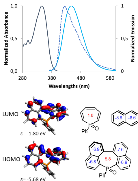
Figure 3: UV-vis absorption (dark blue) and emission (sky blue) in solution and powder (dotted line) of 6 in DCM (up); HOMO and LUMO of 6 calculated at the B3LYP/6-31G**//B3LYP/6-31+G* level (bottom, left); NICS(0) aromaticity patterns of oxa-phosphepine, naphthalene and 6 at the B3LYP/6-311+G**//B3LYP/6-31+G* level (bottom, right).
