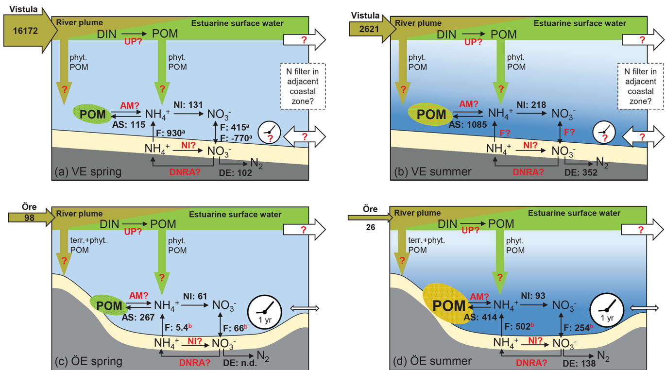
Figure 7. Schematic of the N filter and its driving factors in the Vistula Estuary ( a , b ) and Öre Estuary ( c , d ) in spring and summer. The riverine total N loads are given in tonnes per month in the horizontal brown arrows. The process rates of nitrification (NI), ammonium assimilation (AS), and denitrification (DE), determined in this study, are given in micromoles per square metre per day (volumetric nitrification and ammonium assimilation rates were integrated over the vertical BBL extent to derive areal rates). Benthic POM is fresh but low in concentration in both estuaries in spring (green ellipse), while it is higher in concentration in summer and more degraded in the Öre Estuary (yellow ellipse). Fluxes of \text{NH}_4^+ and \text{NO}_3^- ( F ) in the Vistula Estuary are from Thoms et al. (2018; in situ incubations, a ), and those in the Öre Estuary are from Nedwell et al. (1983; core incubations, not in situ, b ). Other microbial N retention process rates such as N uptake in the surface (UP), benthic ammonification (AM), nitrification (NI), and dissimilatory reduction to ammonia (DNRA) in the sediment are still unknown (marked in red). Fluxes from the Öre Estuary are also marked red, since these fluxes were not measured under in situ conditions; newly measured in situ fluxes are needed for a better evaluation. Also, sedimentation rates of terrestrial and phytoplankton-derived POM from the river (brown arrow) or from the estuarine surface water (green arrow) as well as transport rates (white arrows) and the particle (VE) and nutrient (VE, ÖE) residence time (white clock) are unknown for these two estuaries (red question mark). The conceptual idea of the N filter in the two estuaries is that riverine DIN is supplied to the benthic system indirectly, via POM build-up and sedimentation, which uncouples the peak river N load in spring from enhanced N turnover in the benthic system in summer. In the Öre Estuary, the limited bottom water exchange and hence the long particle residence time results in a high efficiency of the estuarine N filter (see Sect. 4.3). In the Vistula Estuary, the unrestricted bottom topography may lead to transport of DIN and POM with the prevailing alongshore currents and thus to a potential extension of the coastal filter function over a larger area and a longer timescale (see Sect. 4.3). Please note that this figure is not intended to present a closed N budget for these coastal zones.
