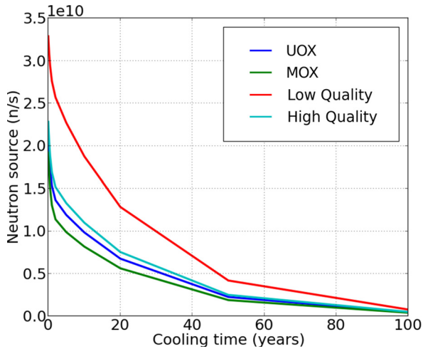
Fig. 5. Comparison of the neutron source per assembly for each of the initial americium feed.
