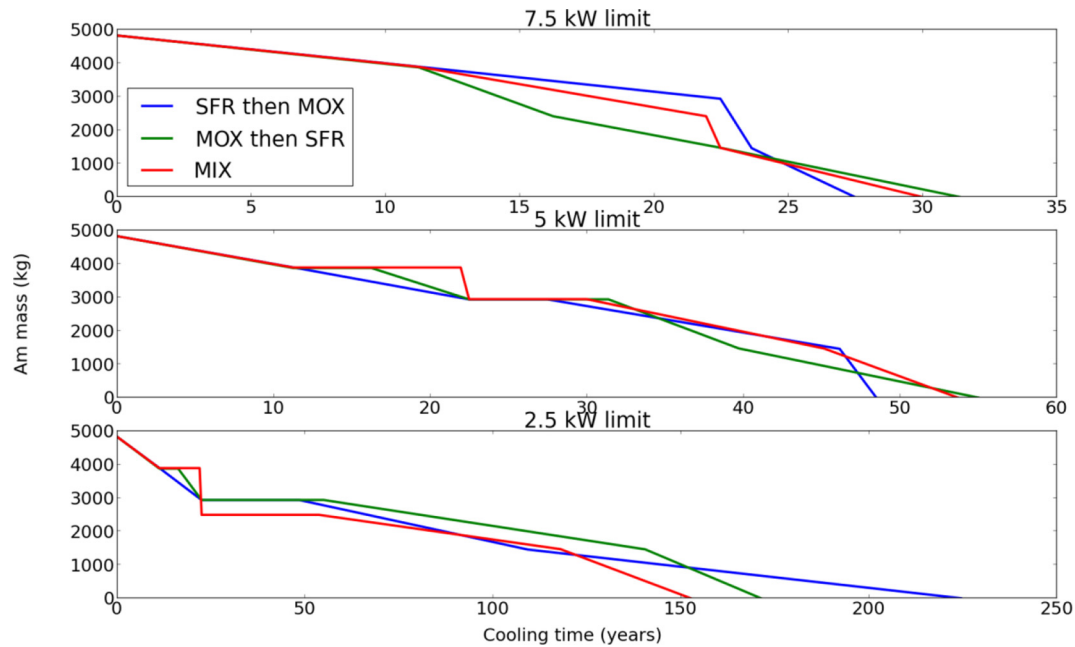
Fig. 3. Evolution of the americium in the fuel cycle depending on the strategy considered and on the reprocessing limit for coupled scenarios with MOX reactors and SFR.
