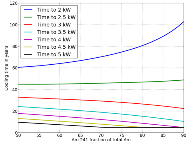
Fig. 2. Cooling time for various limiting values depending on the fraction of ^{241}\text{Am} in the americium isotopic vector. A minimal cooling time of 5 years was considered.
