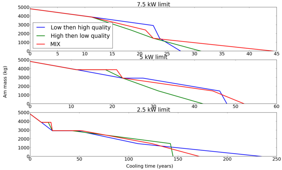
Fig. 4. Evolution of the americium in the fuel cycle depending on the strategy considered and on the reprocessing limit for coupled scenarios with various Pu qualities in SFR.
