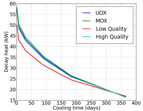
Fig. 6. Comparison of the short term decay heat per assembly for each of the initial americium feed.
