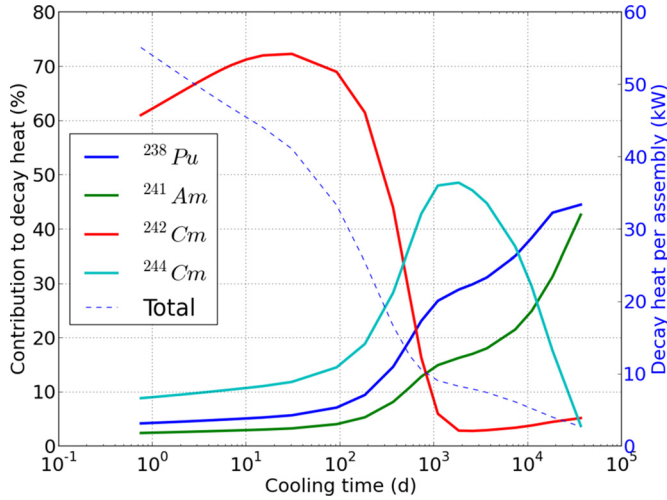
Fig. 1. Evolution of the various contributions to total decay heat versus time.
