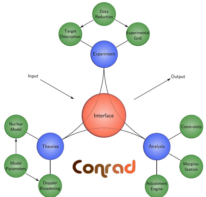
Fig. 2. General overview of the CONRAD code.
