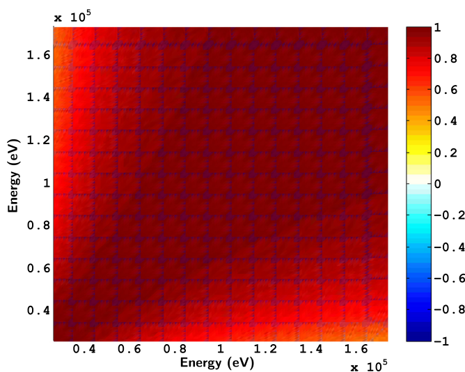
Fig. 3. A priori covariance matrix on ^{238}\text{U} total cross section.
