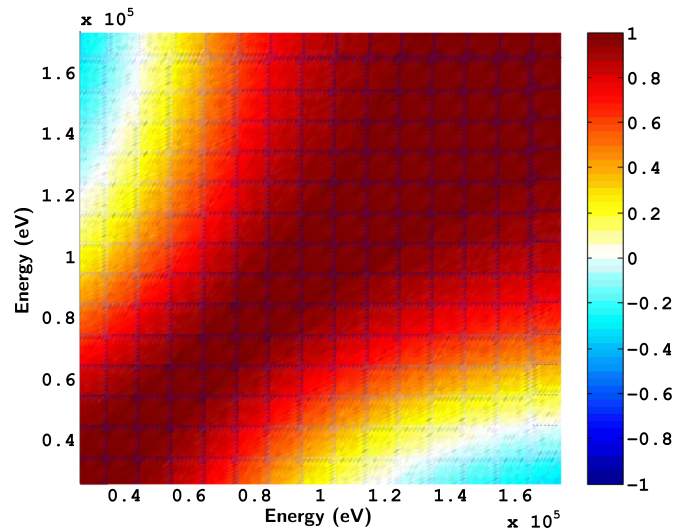
Fig. 4. A posteriori covariance matrix on ^{238}\text{U} total cross section.
