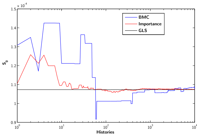
Fig. 6. S_0 mean value convergence.
