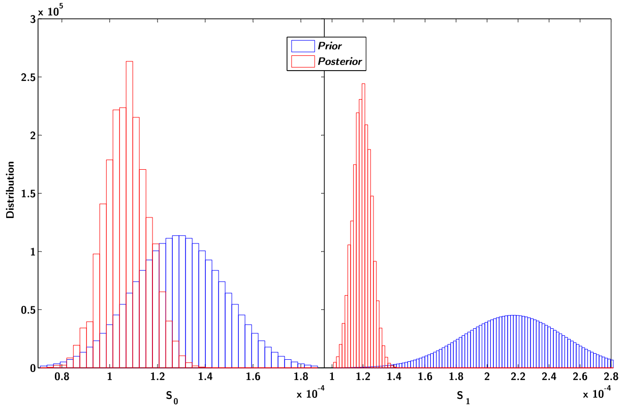
Fig. 5. S_0 and S_1 distributions obtained with the classical BMC method.
