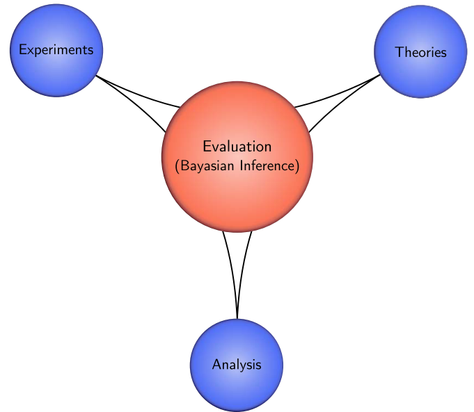
Fig. 1. General overview of the evaluation process.
