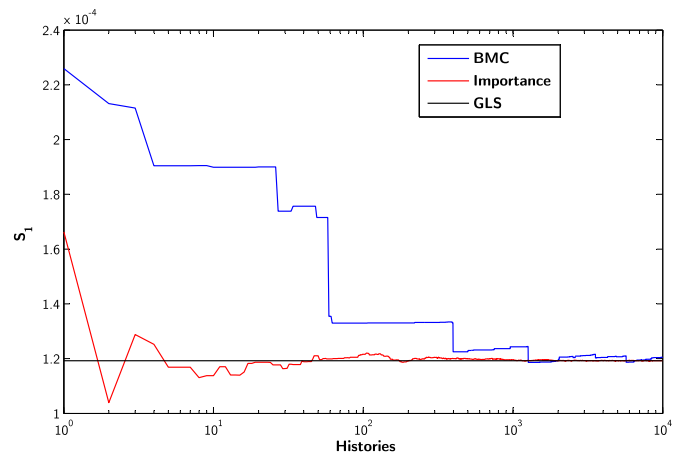
Fig. 7. S_1 mean value convergence.
