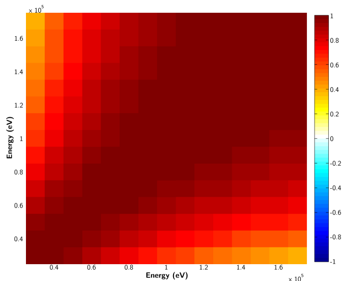
Fig. 8. A posteriori covariance of the ^{238}\text{U} total cross section.
