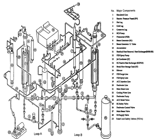
Fig. 1. General view of LSTF [1].
