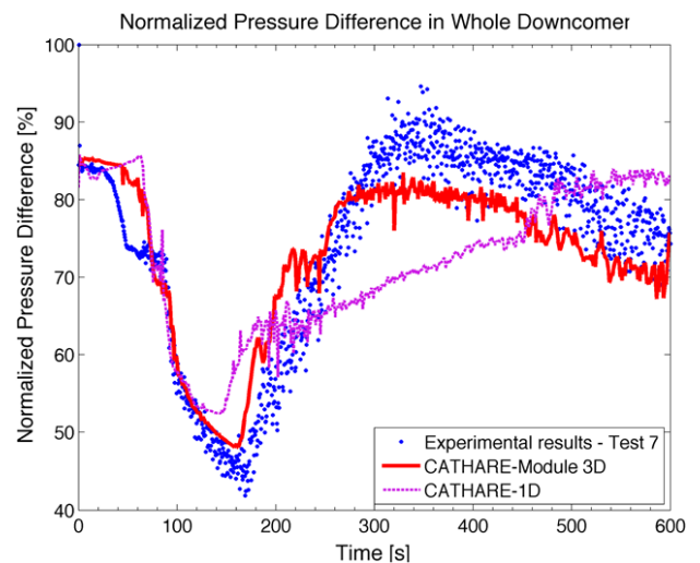
Fig. 10. Pressure difference in whole downcomer.
