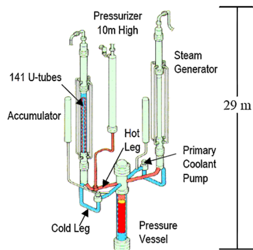
Fig. 2. The view of hot and cold legs in LSTF [2].
