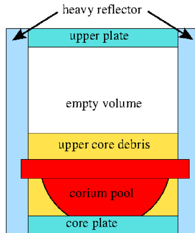
Fig. 2. A simplified core geometry for the corium pool propagation in core. All the core components are presented (upper plate, core support plate, lower and upper core debris, heavy reflector, corium pool [2 shapes], and empty volume).
