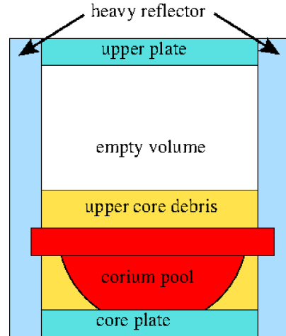
Fig. 2. A simplified core geometry for the corium pool propagation in core. All the core components are presented (upper plate, core support plate, lower and upper core debris, heavy reflector, corium pool [2 shapes], and empty volume).
