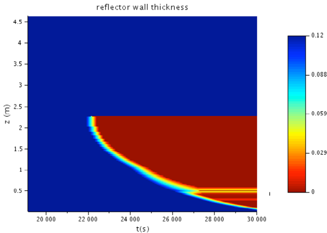
Fig. 5. Variation of the reflector thickness (in m) depending on the level (in m) from the core support plate and during time (in s). Two reflector ruptures occur (first at 2.26 m and second at 0.5 m).
