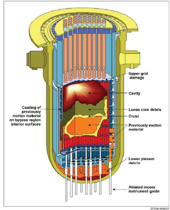
Fig. 1. Scheme of the lower head and core final state of the TMI-Unit2 severe accident.
