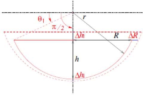
Fig. 3. Radial and axial expansion of a spherical cap associated with the corium pool.
