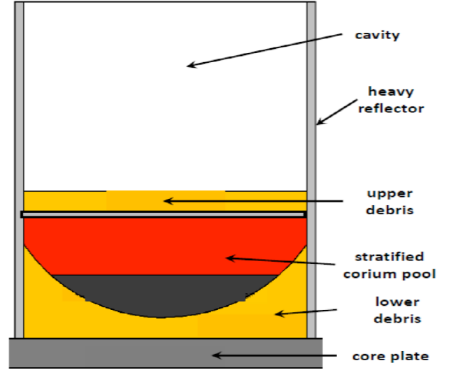
Fig. 4. Example of corium pool propagation in core computed with the simplified geometrical model in the PROCOR framework (computation results). The corium pool is stratified: the layers from bottom to top are: a heavy metal layer ( m = 20,875 kg, T = 3090 K), an oxidic layer ( m = 70,389 kg, T = 3139 K), a steel layer ( m = 571 kg, T = 2219 K). The corium pool shape is formed by a spherical cap and a cylinder.
