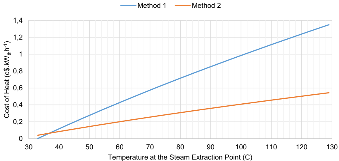
Fig. 7. Cost of heat vs. temperature at the steam extraction point.
