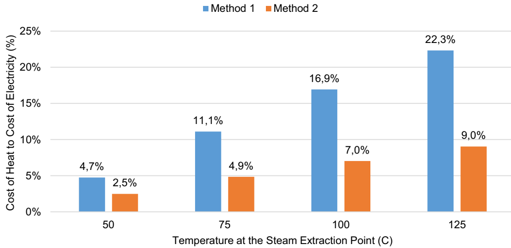
Fig. 8. Cost of heat to cost of electricity vs. temperature at the steam extraction point.
