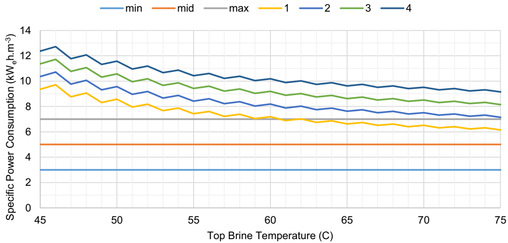
Fig. 13. MED energy cost vs. top brine temperature. Based on Method 1. 1, 2, 3, 4: MED specific electric consumption equal to 1, 2, 3 and 4 \text{kW}_e \text{m}^{-3} respectively. min, mid, and max: minimal, medium and maximal specific electric consumption of the SWRO process as reported in literature.
