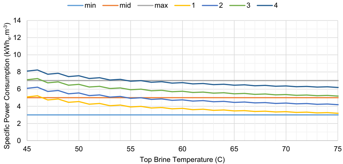
Fig. 14. MED energy cost vs. top brine temperature. Based on Method 2. 1, 2, 3, 4: MED specific electric consumption equal to 1, 2, 3 and 4 \text{kW}_e \text{m}^{-3} respectively. min, mid, and max: minimal, medium and maximal specific electric consumption of the SWRO process as reported in literature.
