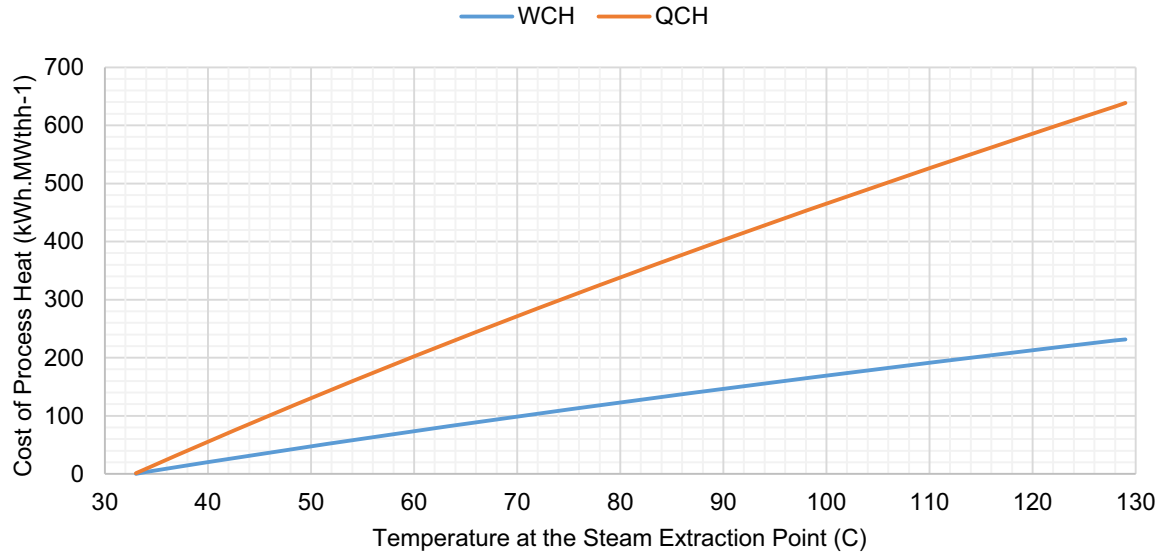
Fig. 5. WCH and QCH vs. temperature at the steam extraction point.
