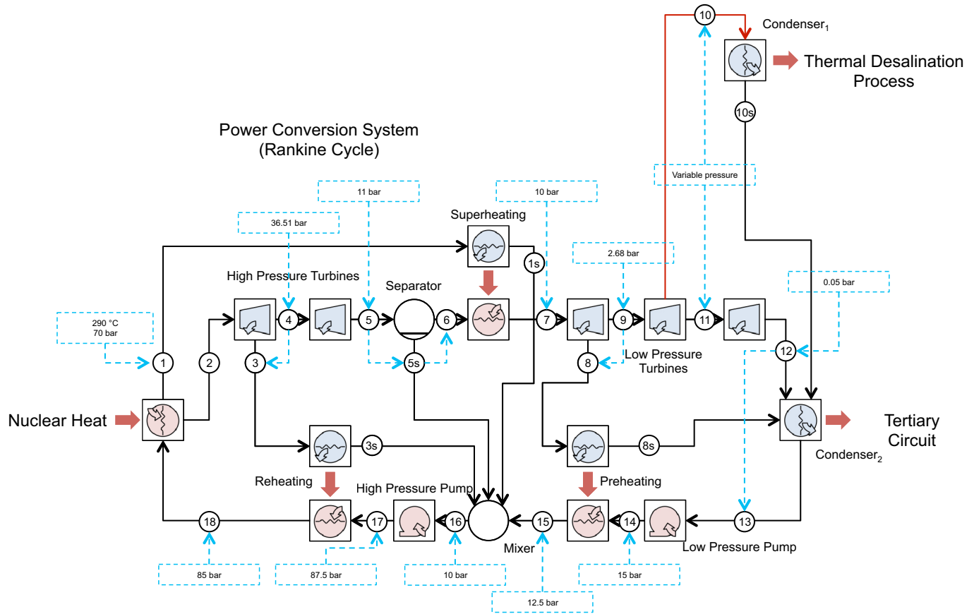
Fig. 2. Power conversion system architecture.
