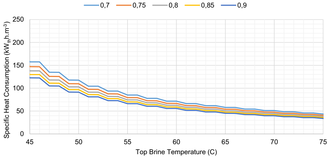
Fig. 12. MED specific thermal power consumption vs. top brine temperature. 0.7, 0.75, 0.8, 0.85, 0.9: GOR to number of stages.
