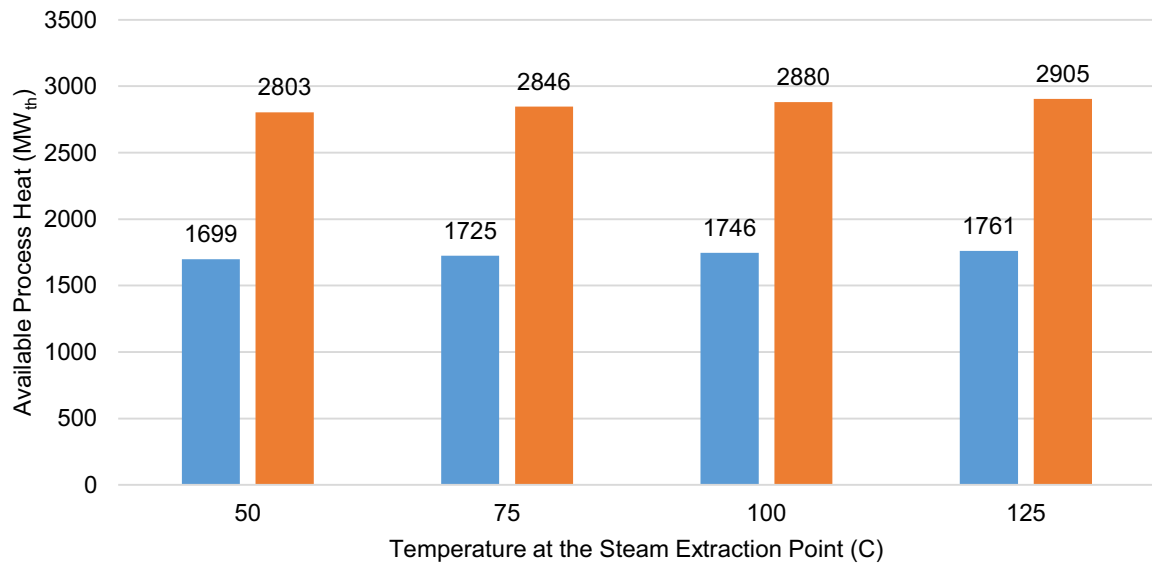
Fig. 4. Available heat for the external process vs. temperature at the steam extraction point. Blue bar: PWR 1000 MWe (2748 MW th ); orange bar: PWR 1650 MWe (4534 MW th ).
