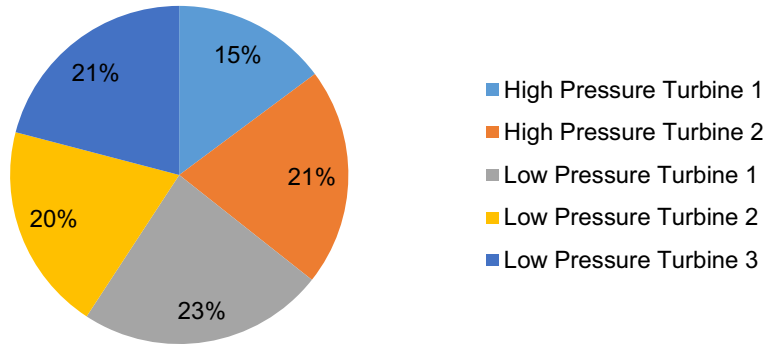
Fig. 3. Contribution of steam turbines to SPP's electricity output.
