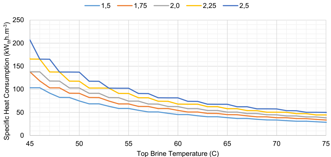
Fig. 11. MED specific thermal power consumption vs. top brine temperature. 1.5, 1.75, 2.0, 2.25, 2.5: average temperature drop between stages ( ^{\circ}\text{C} ).
