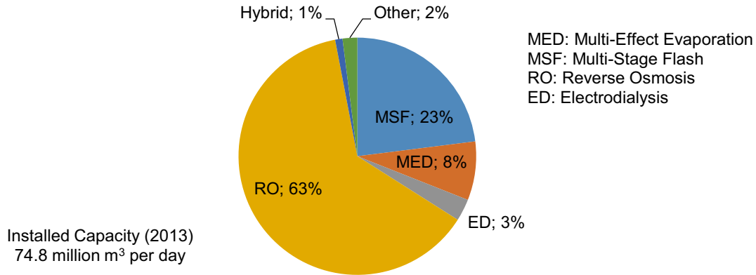
Fig. 1. Total worldwide installed capacity by technology.
