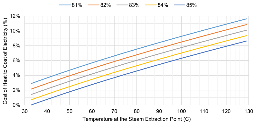
Fig. 10. Cost of heat to cost of electricity vs. temperature at the steam extraction point (Method 2) for different values of (\text{DPP}_2) availability.
