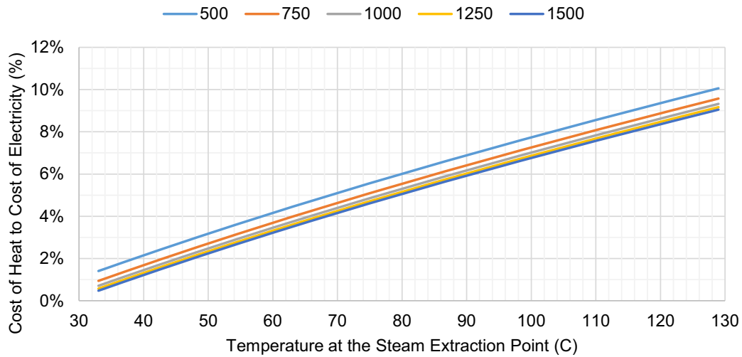
Fig. 9. Cost of heat to cost of electricity vs. temperature at the steam extraction point (Method 2) for different values of process thermal power ( \text{MW}_{\text{th}} ).
