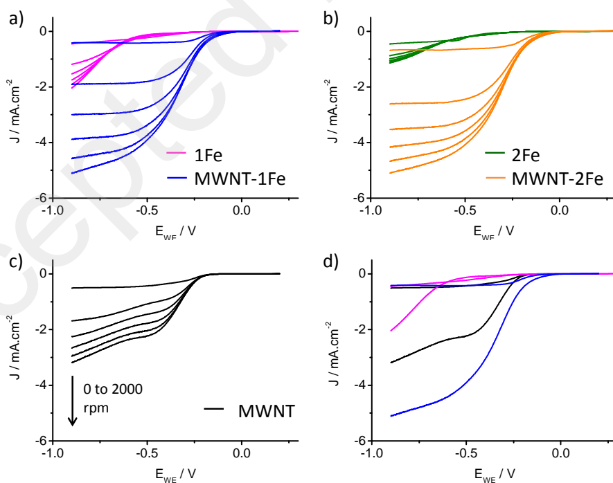
Figure 4. Polarization curves at different rotation rates (0, 400, 800, 1200, 1600 and 2000 rpm) recorded for ORR in \text{O}_2 -saturated at pH 10 (phosphate buffer solution) (scan rate = 5 mV/s, room temperature) on GC with predeposited (a) 1Fe (pink) and MWNT-1Fe (blue); (b) 2Fe (green) and MWNT-2Fe (orange); (c) MWNT (black). (d) Comparison between MWNT , MWNT-1Fe and 1Fe at 0 and 2000 rpm.
