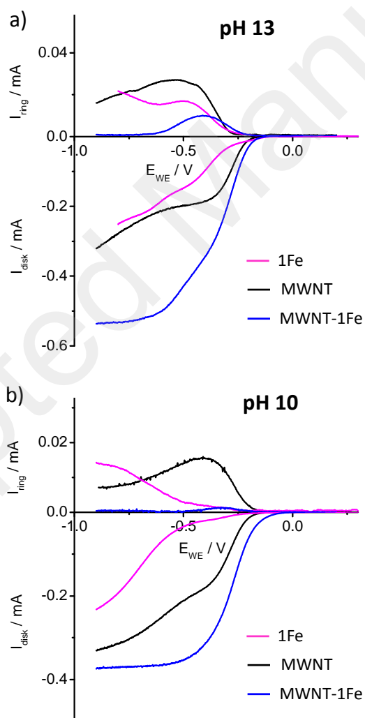
Figure 5. RRDE measurements of oxygen reduction (negative current) and hydrogen peroxide oxidation (positive current) for MWNT (black), 1Fe (pink) and MWNT-1Fe (blue) at (a) pH 13 and (b) pH 10 in \text{O}_2 -saturated solutions. The ring electrode was polarized at 0.260 V vs Ag/AgCl. Rotation rate: 400 rpm; scan rate: 5 \text{mV s}^{-1} .
