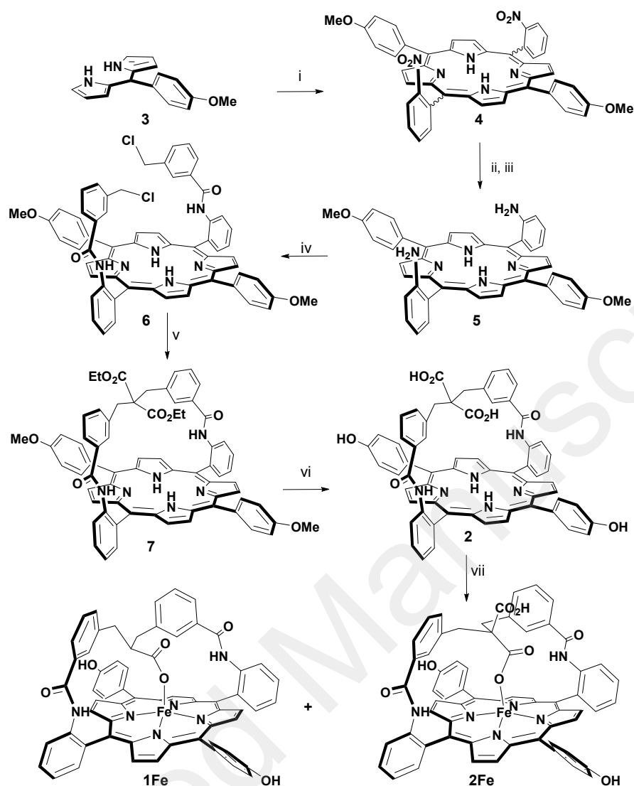
Scheme 1. Synthesis of iron porphyrins 1Fe and 2Fe bearing one and two overhanging carboxylic acid groups respectively, for MWNT coating. (i) 2-nitrobenzaldehyde, \text{CH}_2\text{Cl}_2 , \text{BF}_3\text{-Et}_2\text{O} , 2 h, then DDQ, 20%; (ii) \text{SnCl}_2 , HCl, 80%; (iii) silica gel chromatography, \text{CH}_2\text{Cl}_2 , 66%; (iv) 3-(chloromethyl)benzoyl chloride (3 eq), \text{NEt}_3 , THF, 85%; (v) \text{CH}_2(\text{CO}_2\text{Et})_2 (10 equiv.), THF, EtONa, room temp., 12 h, 80%; (vi) \text{BBr}_3 , \text{CH}_2\text{Cl}_2 , room temp., 12 h, 80%; (vii) \text{FeBr}_2 , 2,6-lutidine, THF, reflux overnight, silica gel column chromatography after air oxidation and HCl (1M) washing, 1Fe (41%), 2Fe (37%).
