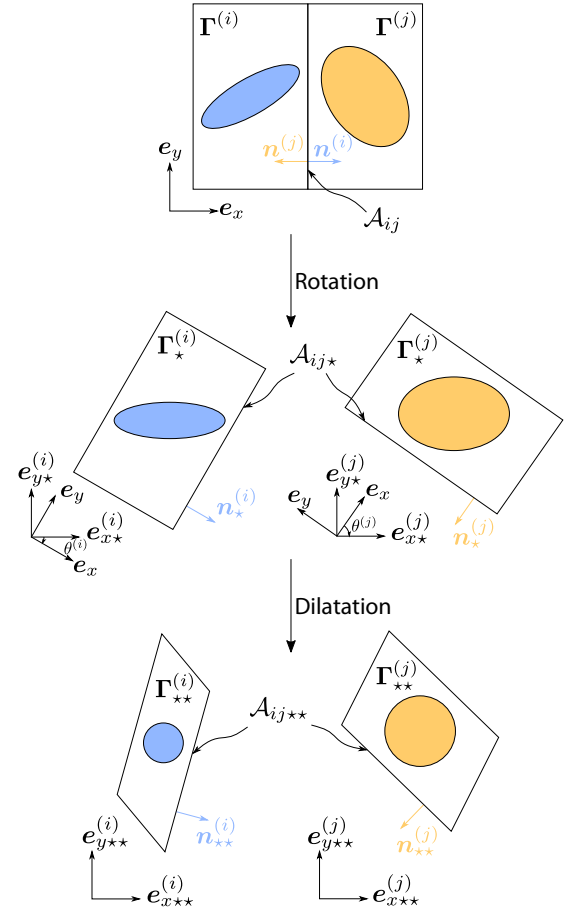
FIG. 3. Illustration of the two successive transformations (rotation and dilatation) applied to two adjacent tiles for the BEM flow solution in an anisotropic multidomain.
