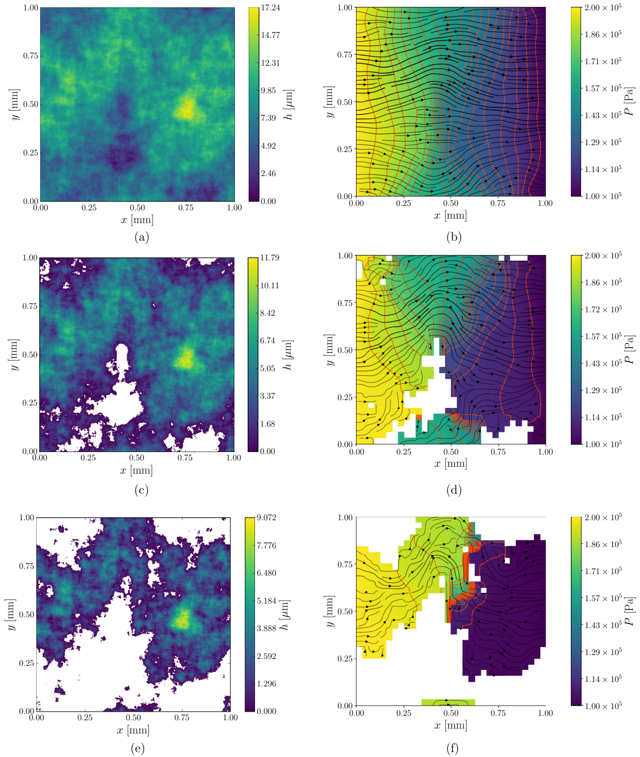
FIG. 11. Left: Aperture field of the fractal surface at different squeezing displacement w/R_t = 0.00 ( \overline{Kn} \approx 0.015 ) (a); w/R_t = 0.32 ( \overline{Kn} \approx 0.041 ) (c); and w/R_t = 0.47 ( \overline{Kn} \approx 0.17 ) (e). White zones denote contact spots of zero aperture. Right: Color map of the computed pressure fields with superimposed isobar lines (in orange) and mass flux streamlines (arrow lines) computed with the two-scale method for the corresponding aperture fields on the left. (b) w/R_t = 0.00 ( \overline{Kn} \approx 0.015 ); (d) w/R_t = 0.32 ( \overline{Kn} \approx 0.041 ) (f) w/R_t = 0.47 ( \overline{Kn} \approx 0.17 ). 32 \times 32 tessellation. White zones denote nonpercolating tiles.
