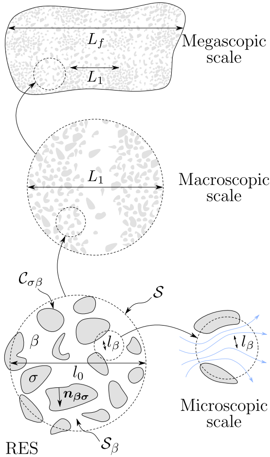
FIG. 1. Schematic view of the different scales of the fracture for the problem. \beta is the fluid phase and the contact zones are denoted by \sigma . Note that the only length-scale constraint is l_\beta \ll L_1 .
