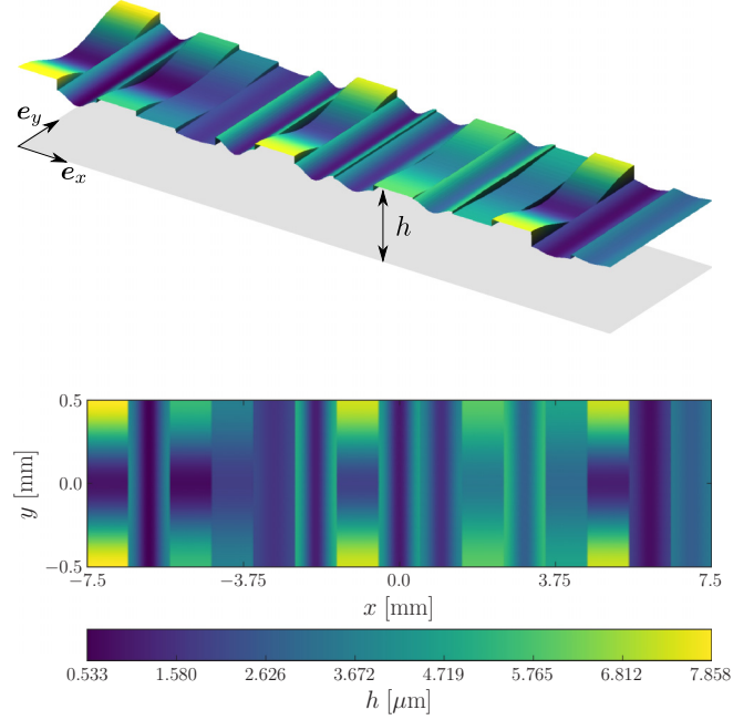
FIG. 4. Aperture field h(x, y) of the synthetic surface composed of 15 “cosine tiles” of variable parameters. The serial configuration corresponds to the flow along \mathbf{e}_x . Top: 3D view. Bottom: 2D top view. Aspect ratio is distorted for clarity of presentation.
