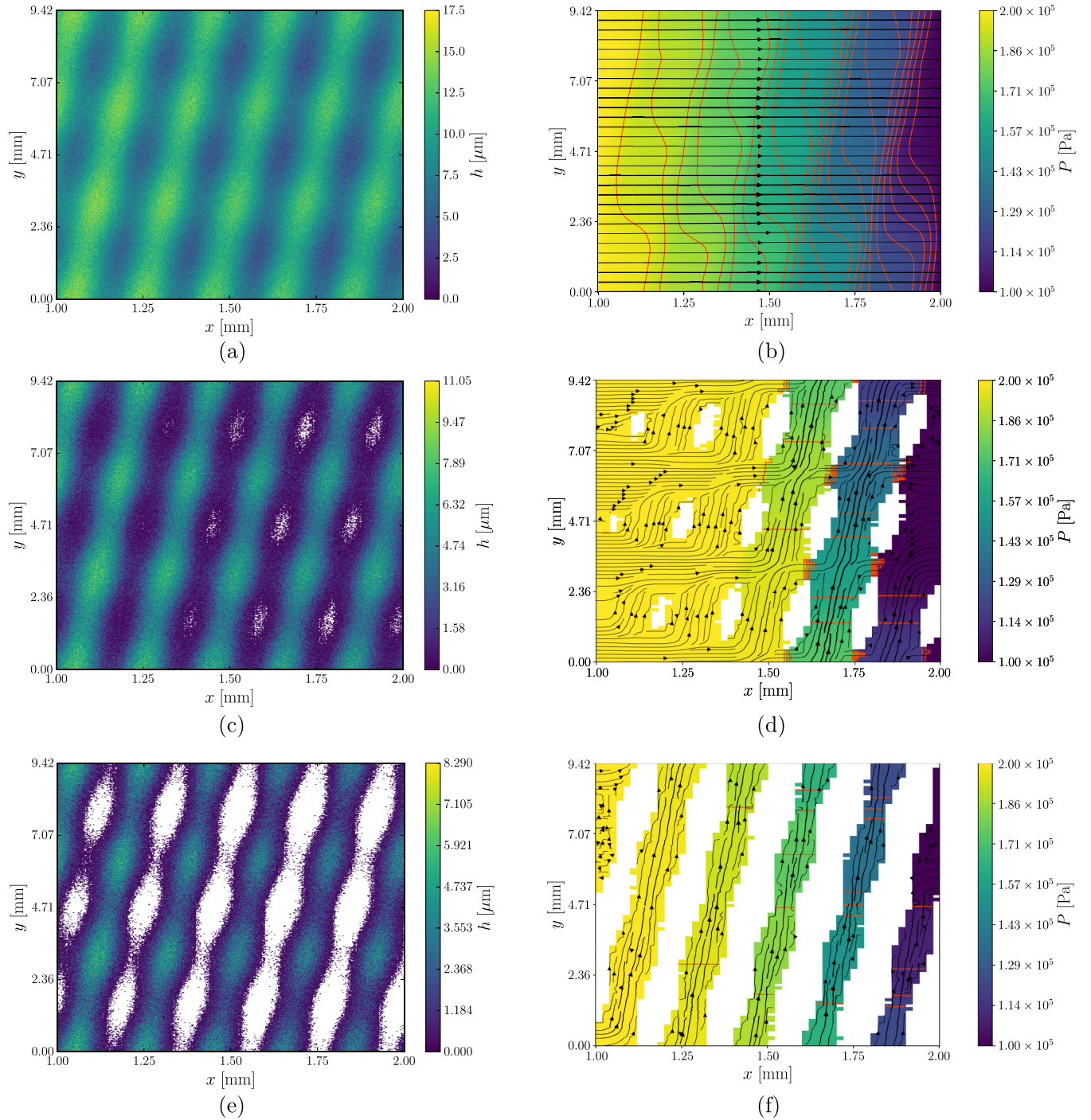
FIG. 9. Left: Aperture field of the spiral-groove surface at different squeezing displacement w/R_t = 0.00 ( \overline{\text{Kn}} \approx 0.015 ) (a); w/R_t = 0.37 ( \overline{\text{Kn}} \approx 0.37 ) (c); and w/R_t = 0.53 ( \overline{\text{Kn}} \approx 1.68 ) (e). White zones denote contact spots of zero aperture. Right: Color map of the computed pressure fields with superimposed isobar lines (in orange) and mass flux streamlines (arrow lines) computed with the two-scale method for the corresponding aperture fields on the left. (b) w/R_t = 0.00 ( \overline{\text{Kn}} \approx 0.015 ); (d) w/R_t = 0.37 ( \overline{\text{Kn}} \approx 0.37 ); (f) w/R_t = 0.53 ( \overline{\text{Kn}} \approx 1.68 ). 50 \times 96 tessellation. White zones denote nonpercolating tiles. The aspect ratio is distorted for clarity of the representation.
