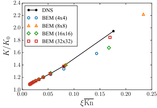
FIG. 12. Dimensionless transmissivity of the fractal surface as a function of the average Knudsen number.
