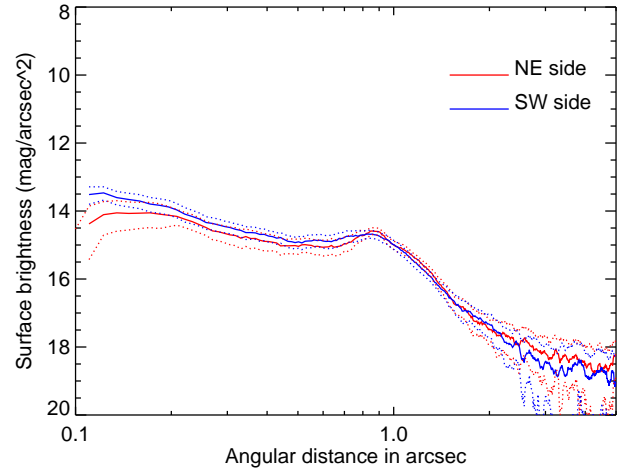
Fig. 11. Surface brightness profile of the disk measured in the IRDIS BB_J DPI Q_0 science image. The blue line represents the SW side of the disk and the red line represents its counterpart on the NE side. The dotted lines represent the error bars.
