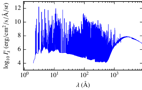
Fig. 16. Specific intensity I_{\lambda}^i emerging from the reverse shock front during the QPO cycle of the Hybrid model (at t = 70 s, see Fig. 14).
