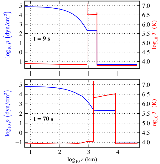
Fig. 13. Snapshots of the temperature (red) and pressure (blue) at 9 s (top) and 70 s (bottom) for the Hybrid case.
