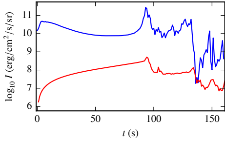
Fig. 17. Time-variation of the 2–27 Å (LTE) integrated X-ray outgoing intensity ( I_X^i , blue) and of the optically thin post-shock emission ( I_A , red) during a QPO cycle for the Hybrid setup.
