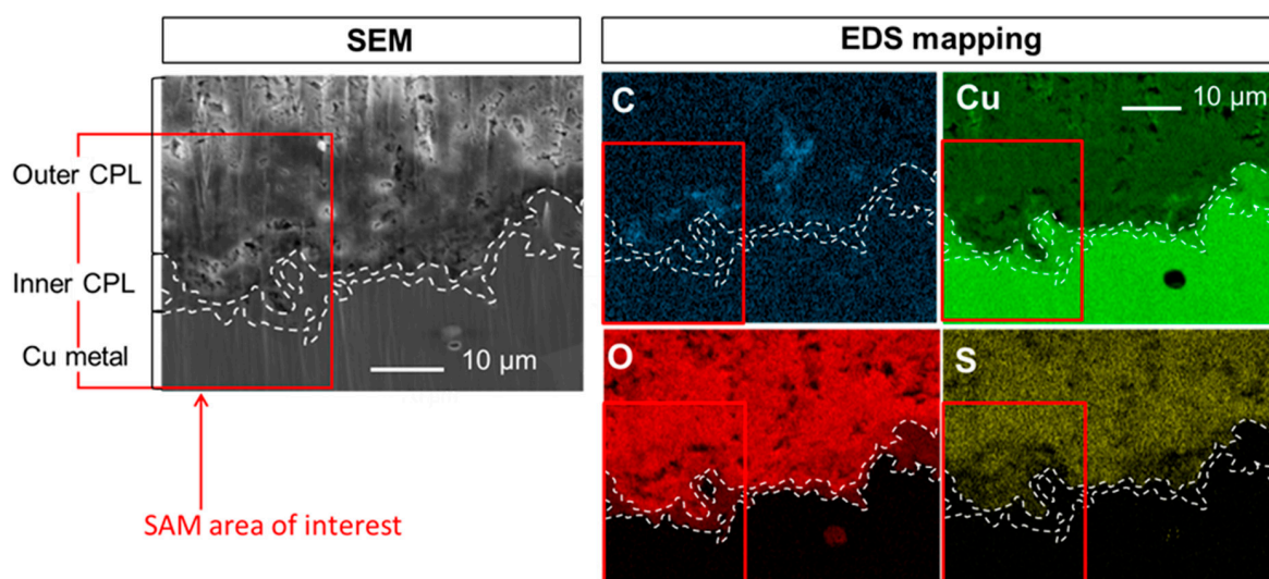
Figure 7. Sample immersed in \text{HC}_{10} for one minute: SEM-EDS elemental mappings of C, Cu, O and S at the CPL/metal interface.
