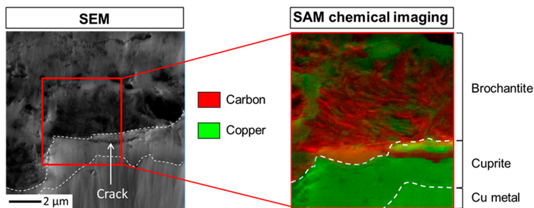
Figure 6. Sample immersed in \text{HC}_{10} for thirty minutes: SEM image and SAM analysis area ( 5.3 \mu\text{m} per 4.9 \mu\text{m} ) (a), overlapping of C and Cu chemical images (b).
