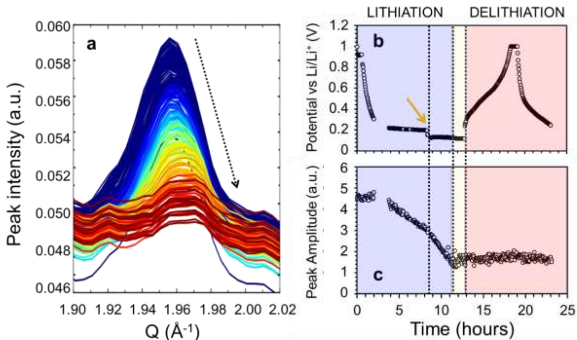
Figure 5 : a) Si-Ge [111] peak intensity variations measured by operando synchrotron XRD during the first lithiation. The peak decreases in intensity (from blue to red) indicating the continuous amorphization of the active particles. b) Voltage against time, with a change in current at ca. 8 hours, indicated by the arrow, and a floating period at the end of the lithiation, materialized by the yellow shadowed area. c) Peak amplitude obtained by a Gaussian fit to the XRD data, as a function of time.
