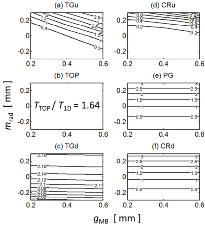
Figure 19. Transient ELM temperature spike (normalized to that of an ideal axisymmetric surface) at OVT MBs having a shallow toroidal-poloidal bevel ( h_{tor}=0.5 mm, h_{pol}=0.5 mm) with the intra-PFU MB alignments varied according to Table 1. The PFUs are poloidally aligned ( m_{pol}=0 mm). For definition of measurement points see Figure 3.
