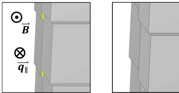
Figure 21. View along magnetic field lines of two OVT PFUs equipped with MBs having a toroidal-poloidal bevel ( h_{\text{tor}}=0.5 mm, h_{\text{pol}}=0.5 mm). The downstream PFU is misaligned radially by m_{\text{PFU}}=0.3 mm and the poloidal gap width is g_{\text{PFU}}=0.7 mm (worst case). In the left panel, the upstream PFU is shifted poloidally m_{\text{pol}}=2 mm upward with respect to its downstream neighbour. The exposed LE is coloured yellow. On the right, the upstream PFU is shifted poloidally m_{\text{pol}}=-2 mm downward with respect to its downstream neighbour.
