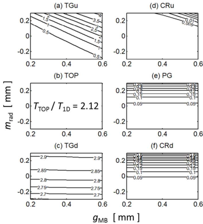
Figure 20. Transient ELM temperature spike (normalized to that of an ideal axisymmetric surface) at OVT MBs having a deep toroidal-poloidal bevel ( h_{tor}=1.1 mm, h_{pol}=0.6 mm) with the intra-PFU MB alignments varied according to Table 1. The PFUs are poloidally aligned ( m_{pol}=0 mm). For definition of measurement points see Figure 3.
