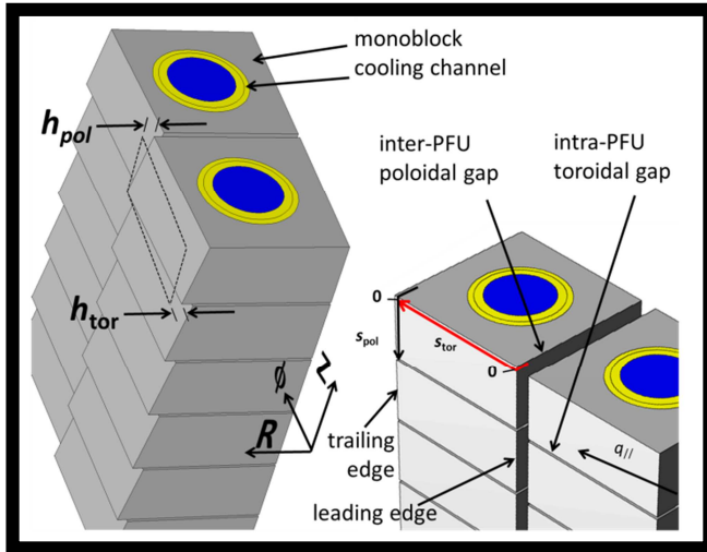
Figure 1. Schematic of two neighbouring PFUs at the OVT. At left, with greatly exaggerated toroidal-poloidal planar beveling for illustration, the dashed rectangle represents the flat surface of a MB before beveling. The planar bevel is characterized by the depths h_{tor} in the toroidal direction, and h_{pol} in the poloidal direction. At right, the poloidal and toroidal gaps, as well as leading and trailing edges are indicated, and the surface coordinates s_{pol} and s_{tor} along which temperature profiles will be plotted throughout this paper are defined.
