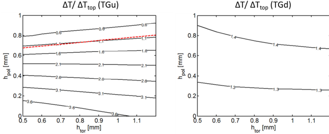
Figure 10. As in Figure 9 now with m_{\text{rad}}=0.3 mm.
