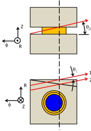
Figure 5. Schematic illustration of why toroidal beveling leads to deeper penetration of magnetic field lines into TGs. The upper diagram represents the frontal view of two MBs on a divertor vertical target separated by a TG. The magnetic field line (red arrow) grazes the lower edge of the upper MB at the position indicated by the dashed line, crosses the TG, and strikes the lower MB at its trailing edge. The lower diagram shows the view along the cooling pipe for the case of (1) an unshaped MB and (2) a toroidally beveled MB.
