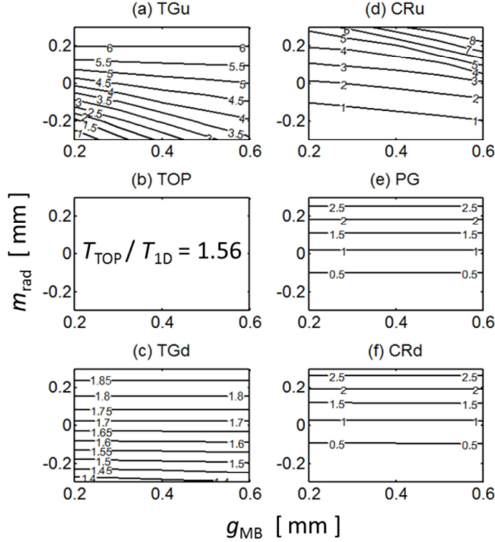
Figure 18. Transient ELM temperature spike (normalized to that of an ideal axisymmetric surface) at OVT MBs having a simple toroidal bevel ( h_{tor}=0.5 mm, h_{pol}=0 mm) with the intra-PFU MB alignments varied according to Table 1. The PFUs are poloidally aligned ( m_{pol}=0 mm). For definition of measurement points see Figure 3.
