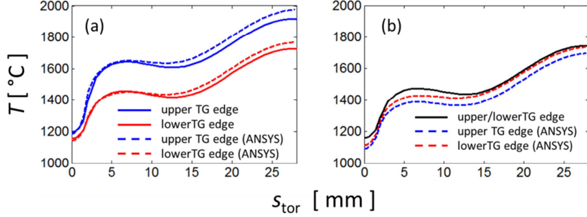
Figure 4. Comparison of the simple finite difference model (full curves) with finite element simulations (dashed) of the true geometry for (a) a simple toroidal bevel and (b) a shallow toroidal-poloidal bevel. In (a) the temperature is shown along the upper (blue curves) and lower (red curves) TG edges. In (b), the upper and lower edge temperatures are equal in the simple model (black curve), while for the ANSYS simulation the upper (blue curve) and lower (red curve) edge temperatures are shown. The toroidal distance along the TG edge is designated s_{\text{tor}} .
