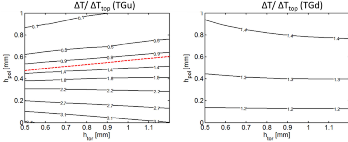
Figure 9. TG edge temperature increase during an ELM with respect to the increase at the top surface (including MB beveling and VT tilting) as a function of toroidal and poloidal bevel depths at OVT upper (left panel) and lower (right panel) edges assuming intra-PFU radial misalignment of m_{\text{rad}}=0.1 mm. The dashed line on the left panel indicates the poloidal bevel depth for which total magnetic shadowing of the TG edge is achieved.
