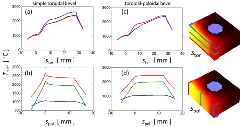
Figure 16. Steady state temperatures at OVT MBs having a simple toroidal bevel ( h_{\text{tor}}=0.5 mm, h_{\text{pol}}=0.0 mm): (a) Toroidal profiles at upper TG edge (blue curves), through the center of the MB (green curves), and at lower TG edge (red curves). (b) Poloidal profiles at poloidal LE (blue curves), through the center of the MB (green curves), and along the trailing poloidal edge (red curves). The same profiles are shown in (c,d) for a MB with toroidal-poloidal bevel ( h_{\text{tor}}=0.5 mm, h_{\text{pol}}=0.5 mm). In both cases g_{\text{MB}}=0.5 mm and m_{\text{rad}}=0.1 mm. The PFUs are poloidally aligned ( m_{\text{pol}}=0 mm).
