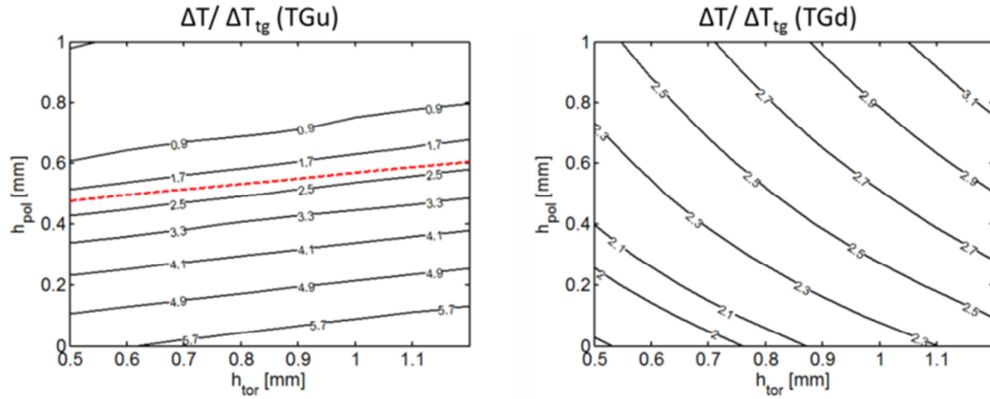
Figure 7. TG edge temperature increase during an ELM with respect to the increase at an ideal axisymmetric target as a function of toroidal and poloidal bevel depths at OVT upper (left panel) and lower (right panel) edges assuming VT tilting angle \Delta\theta=0.5^\circ and intra-PFU radial misalignment of m_{\text{rad}}=0.1 mm. The dashed line on the left panel indicates the poloidal bevel depth for which total magnetic shadowing of the TG edge is achieved.
