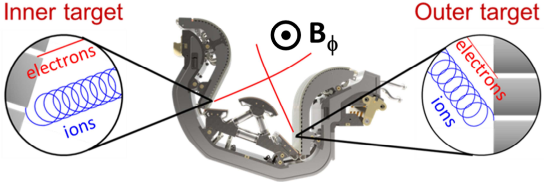
Figure 2. Schematic illustration of an ITER divertor cassette. Due to their Larmor radii being comparable to the gap widths, ions (orbits shown in blue in the insets) strike the upper edges of OVT monoblocks and the lower edges of IVT monoblocks, whereas electrons, strike the upper edges at both targets due to the inclination of the magnetic flux surfaces (red curves). Electrons can be described under the guiding-center approximation, making their orbits equivalent to the red curves. This means that at the IVT, heat loading occurs at both edges of the TGs, whereas at the OVT, only the upper edges are affected. A poloidal bevel can only be effective at the OVT. At the IVT, there is no solution to simultaneously mitigate heating of both edges by poloidal beveling; trying to protect one edge only exposes the other to higher heat flux [7].
