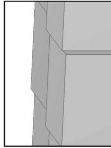
Figure 21. View along magnetic field lines of two OVT PFUs equipped with MBs having a toroidal-poloidal bevel ( h_{\text{tor}}=0.5 mm, h_{\text{pol}}=0.5 mm). The downstream PFU is misaligned radially by m_{\text{PFU}}=0.3 mm and the poloidal gap width is g_{\text{PFU}}=0.7 mm (worst case). In the left panel, the upstream PFU is shifted poloidally m_{\text{pol}}=2 mm upward with respect to its downstream neighbour. The exposed LE is coloured yellow. On the right, the upstream PFU is shifted poloidally m_{\text{pol}}=-2 mm downward with respect to its downstream neighbour.
