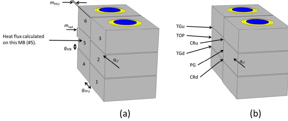
Figure 3. (a) Illustration of the simulation geometry with definitions of intra-PFU and inter-PFU radial steps ( m_{rad} and m_{PFU} respectively) and TG and PG widths ( g_{MB} and g_{PFU} respectively). (b) Definition of heat flux/temperature measurement points on the target MB#5 on which the heat loads are calculated as a function of shadowing by its five neighbours. TGu=upper or "upstream" toroidal gap edge; TOP=the principal exposed surface at the center of the trailing poloidal edge; TGd=lower or "downstream" toroidal gap edge; CRu=upper corner of the PG LE; PG=center of the leading poloidal edge; CRd=lower corner of the PG edge.
