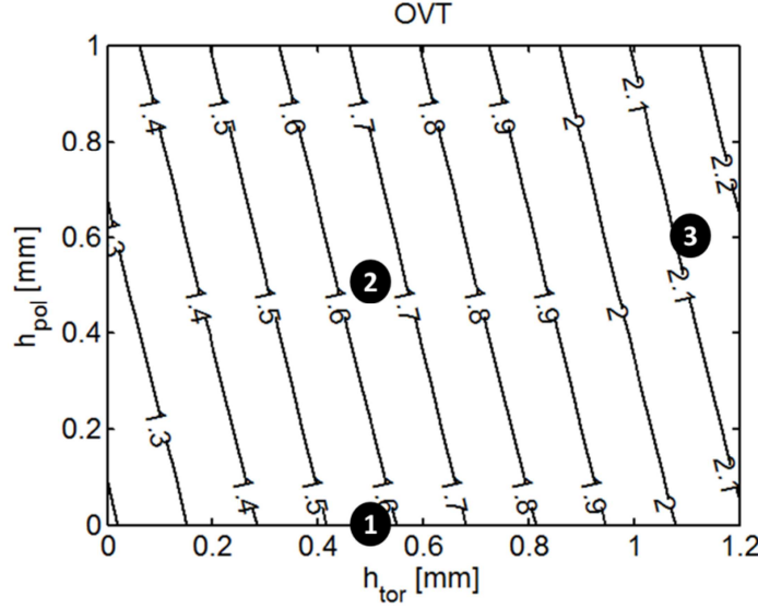
Figure 6. Relative increase of heat flux to MB top surfaces as a function of toroidal and poloidal bevels assuming VT tilting angle \Delta\theta=0.5^\circ . Numbered circles indicate (1) the reference simple toroidal bevel, (2) the shallow and (3) the deep toroidal-poloidal bevels examined in this paper.
