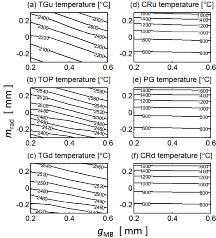
Figure 15. Steady state temperatures at OVT MBs having a shallow toroidal-poloidal bevel ( h_{\text{tor}}=0.5 mm, h_{\text{pol}}=0.5 mm) with the intra-PFU MB alignments varied according to Table 1. The PFUs are poloidally aligned ( m_{\text{pol}}=0 mm). For definition of measurement points see Figure 3.
