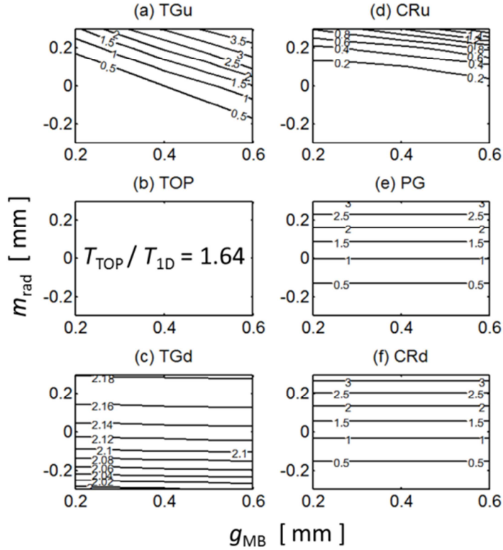
Figure 19. Transient ELM temperature spike (normalized to that of an ideal axisymmetric surface) at OVT MBs having a shallow toroidal-poloidal bevel ( h_{\text{tor}}=0.5 mm, h_{\text{pol}}=0.5 mm) with the intra-PFU MB alignments varied according to Table 1. The PFUs are poloidally aligned ( m_{\text{pol}}=0 mm). For definition of measurement points see Figure 3.
