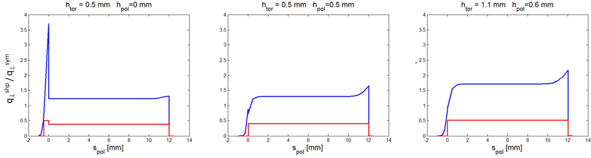
Figure 11. Poloidal profiles along an OVT MB (assuming worst case misalignment with respect to its neighbours, see Table 1) of ion (blue curves) and electron (red curves) ELM heat flux for the reference simple toroidal bevel (left panel), shallow toroidal-poloidal bevel (middle panel), and the deep toroidal-poloidal bevel (right panel). The surface coordinate s_{\text{pol}} runs from inside the upper TG poloidally down the MB to the lower TG. The upper MB edge is at s_{\text{pol}}=0 and the lower edge is at s_{\text{pol}}=12 mm (see Figure 1). Heat flux is expressed in terms of that ( q_{\perp}^{\text{sym}} ) to a smooth, axisymmetric target with no shaping for given plasma parameters.
