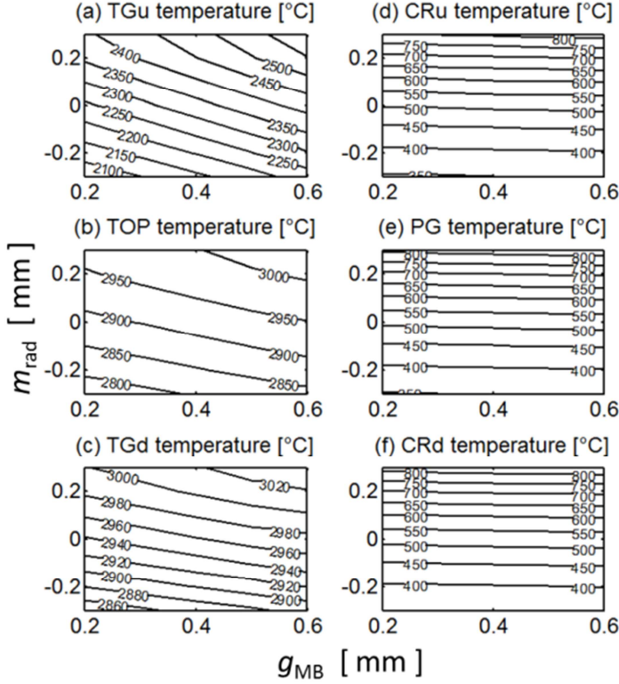
Figure 17. Steady state temperatures at OVT MBs having a deep toroidal-poloidal bevel ( h_{\text{tor}}=1.1 mm, h_{\text{pol}}=0.6 mm) with the intra-PFU MB alignments varied according to Table 1. The PFUs are poloidally aligned ( m_{\text{pol}}=0 mm). For definition of measurement points see Figure 3.
