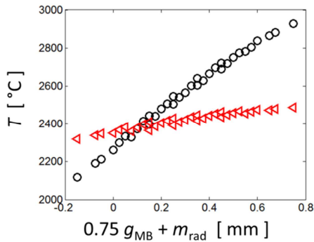
Figure 14. Upper (black circles) and lower (red triangles) TG edge temperature as a function of field line penetration depth into the TG for a simple toroidal bevel ( h_{\text{tor}} = 0.5 , h_{\text{pol}} = 0 ). All the data from Figure 13a,c are plotted.
