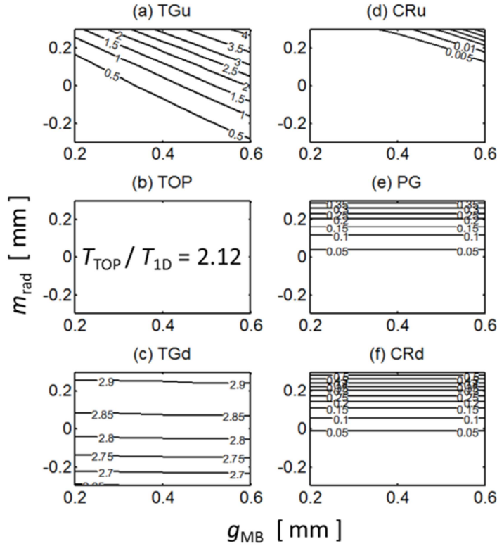
Figure 20. Transient ELM temperature spike (normalized to that of an ideal axisymmetric surface) at OVT MBs having a deep toroidal-poloidal bevel ( h_{\text{tor}}=1.1 mm, h_{\text{pol}}=0.6 mm) with the intra-PFU MB alignments varied according to Table 1. The PFUs are poloidally aligned ( m_{\text{pol}}=0 mm). For definition of measurement points see Figure 3.
