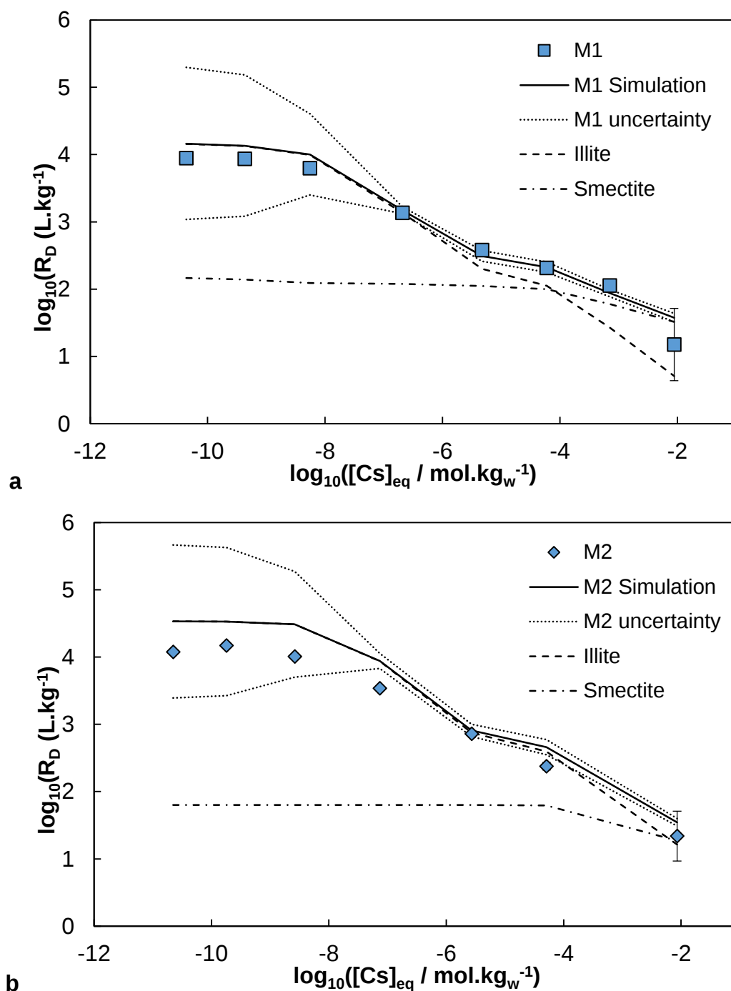
Fig. 6. Adsorption isotherms in equilibrium concentration of Cs at I = 0.1 \text{ mol.kg}_w^{-1} (NaCl), pH = 7 and S/L ratio = 3.8 \text{ g.L}^{-1} on mixture M1 (a) and M2 (b) (composition in Table 2) with the associated simulations (plain) and uncertainty ( 1\sigma , dot), compared with illite (dash) and smectite (dash-dot) contributions.
