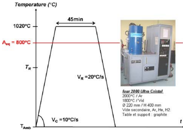
Fig. 1a: Austenization heat treatment
